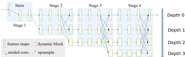
Fig. 4: HRNet architecture.
