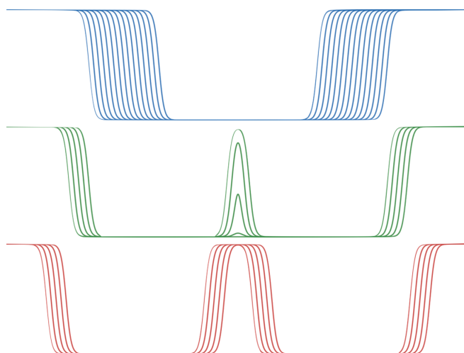
Figure 1. Functional form of C_{\text{double}}(z) illustrating the membrane profile for three regimes of m . High values schematize the aqueous solvent, low values the membrane core. In blue, profiles \forall m \in [0, 13.5] . In green, profiles \forall m \in [13.5, 18] . In red, profiles \forall m > 18 .
