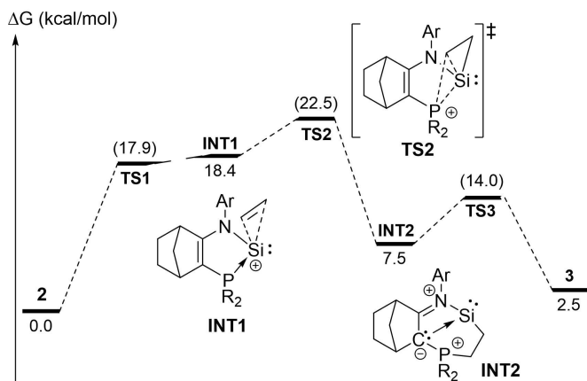
Figure 3. Calculated pathway for the silacyclopropyl cation-silylene interconversion in \text{C}_6\text{H}_5\text{F} . Gibbs energies of intermediates (and transition states) are in \text{kcal mol}^{-1} .
