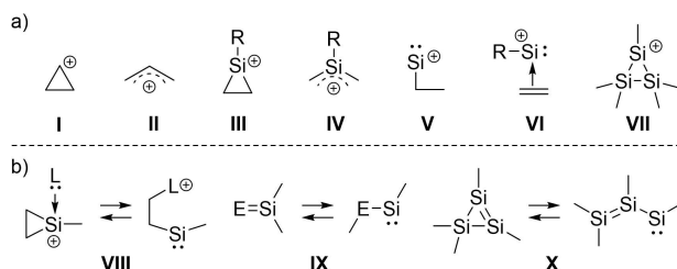
Figure 1. a) Cyclopropenium cation I and allyl cation isomer II and related silicon-containing species ( III–VII ). b) Known reversible silylene isomerizations ( VIII–X ).
