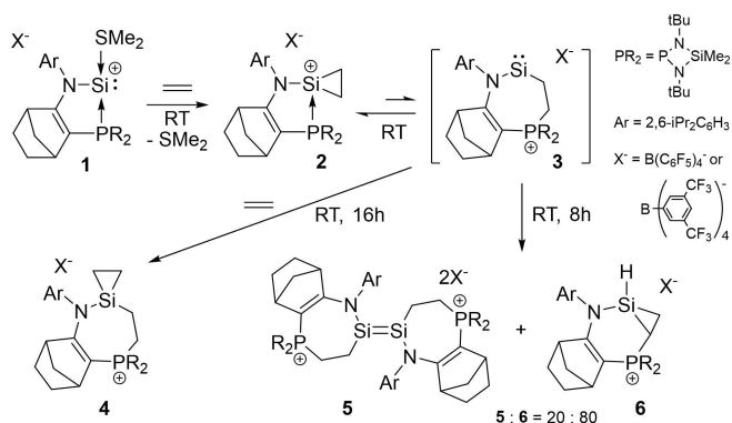
Scheme 1. The synthesis of silacyclopropyl cation 2 , its reversible isomerization to cyclic silylene 3 and the trapping reaction of 3 with ethylene as well as its evolution by dimerization and C–H insertion.
