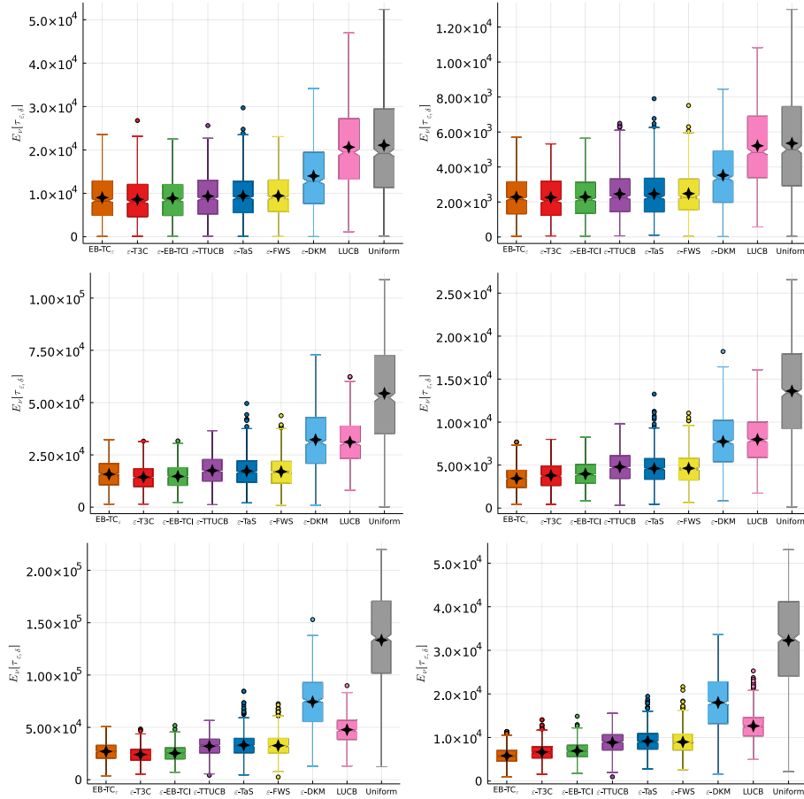
Figure 9: Empirical stopping time on random instances with stopping rule (3) using (left) (\varepsilon, \delta) = (0.05, 0.01) and (right) (\varepsilon, \delta) = (0.1, 0.01) with (top) K = 5 , (middle) K = 10 and (bottom) K = 20 . The BAI algorithms T3C, EB-TCI, TTUCB, TaS, FWS, DKM are modified for \varepsilon -BAI.
