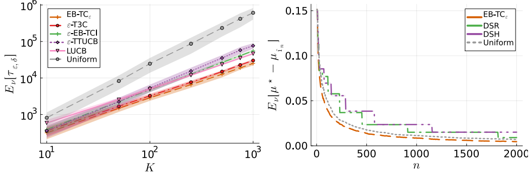
Figure 2: (a) Empirical stopping time on “ \alpha = 0.3 ” instances for varying K and stopping rule (3) using (\epsilon, \delta) = (0.1, 0.01) . The BAI algorithms T3C, EB-TCI and TTUCB are modified to be \epsilon -BAI ones. (b) Empirical simple regret on instance \mu = (0.6, 0.6, 0.55, 0.45, 0.3, 0.2) , in which \text{EB-TC}_{\epsilon_0} with slack \epsilon_0 = 0.1 and fixed \beta = 1/2 is used.
