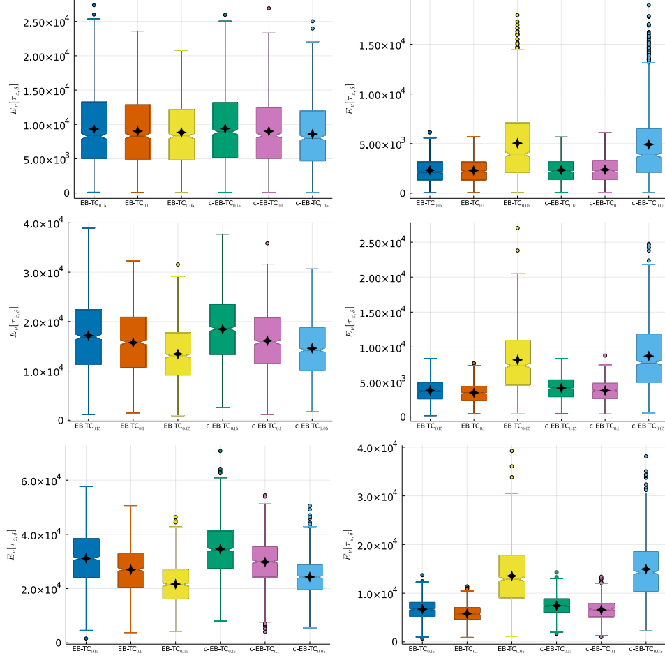
Figure 5: Empirical stopping time on random instances with stopping rule (3) using (left) (\epsilon, \delta) = (0.05, 0.01) and (right) (\epsilon, \delta) = (0.1, 0.01) with (top) K = 5 , (middle) K = 10 and (bottom) K = 20 . “c-” denotes fixed \beta = 1/2 , without refers to IDS.
