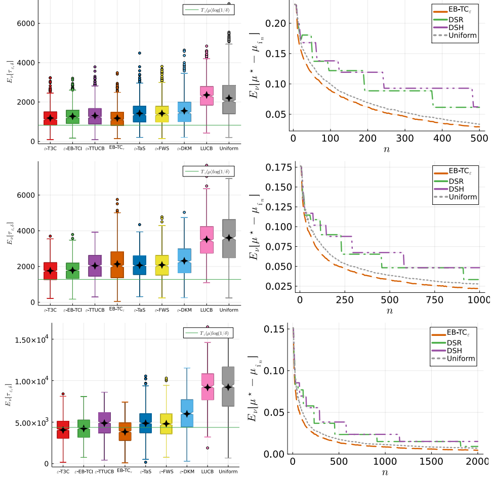
Figure 10: (Left) Empirical stopping time for the stopping rule (3) using \delta = 0.01 and (right) empirical simple regret on instances (top) \mu_1 with \varepsilon = 0.1 , (middle) \mu_2 with \varepsilon = 0.15 and (bottom) \mu_3 with \varepsilon = 0.1 . The BAI algorithms T3C, EB-TCI, TTUCB, TaS, FWS, DKM are modified to be \varepsilon -BAI ones.
