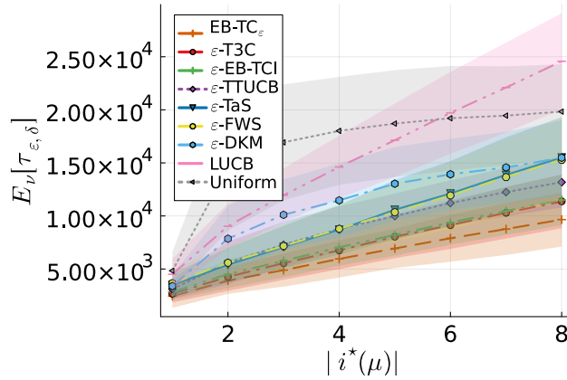
Figure 11: Empirical stopping time with stopping rule (3) using (\varepsilon, \delta) = (0.1, 0.01) on instances \mu \in \{0.6, 0.4\}^{10} for varying |i^*(\mu)| . The BAI algorithms T3C, EB-TCI, TTUCB, TaS, FWS, DKM are modified to be \varepsilon -BAI ones.
