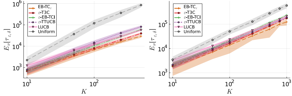
Figure 8: Empirical stopping time on (a) “ \alpha = 0.6 ” instances and (b) “sparse” instances for varying K and stopping rule (3) using (\varepsilon, \delta) = (0.1, 0.01) . The BAI algorithms T3C, EB-TCI and TTUCB are modified to be \varepsilon -BAI ones.
