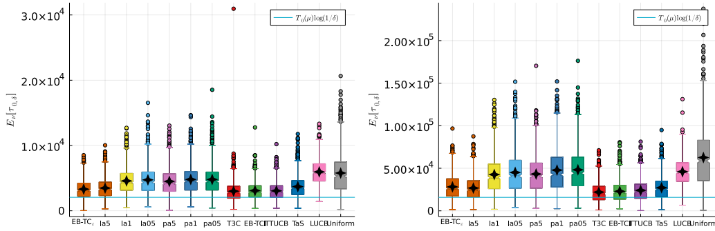
Figure 15: Empirical stopping time for the stopping rule (3) using (\varepsilon, \delta) = (0, 0.01) on instances (a) \mu_1 and (b) \mu_2 . “I” denotes \varepsilon_n = \log(n)^{-\alpha/2} , “p” denotes \varepsilon_n = n^{-\alpha/2} .
