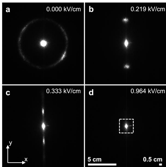
Figure 6. Laser diffraction pattern taken using the experimental setup ES4 (the AC electric field is applied in the x direction), showing the alignment of the CNC suspension at low to moderate electric fields, before the instability is observed. a) initial diffraction pattern from the polydomain cholesteric structure at rest, b) pattern indicating the reorientation of the helicoidal domains, c) distortion and unwinding of the cholesteric structure, d) completely unwound structure into a nematic order. The distance from sample to screen was z_s = 15 cm and the scale bar indicates the distances on screen (e.g., 5 cm corresponds to q \approx 3.18 \mu\text{m}^{-1} , or
