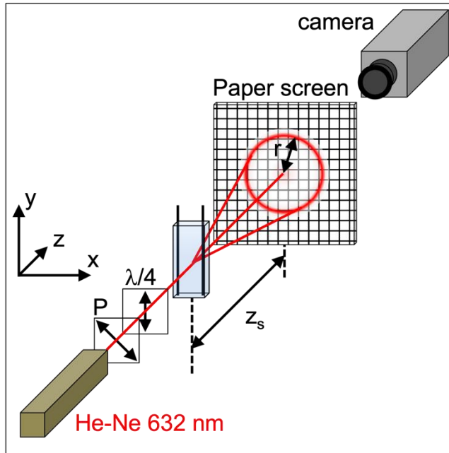
Figure 2. Schematics describing the experimental setup ES4 for the observation of the laser diffraction pattern under electric fields. The distance z_s was varied to access different ranges of scattering vector on the screen.
