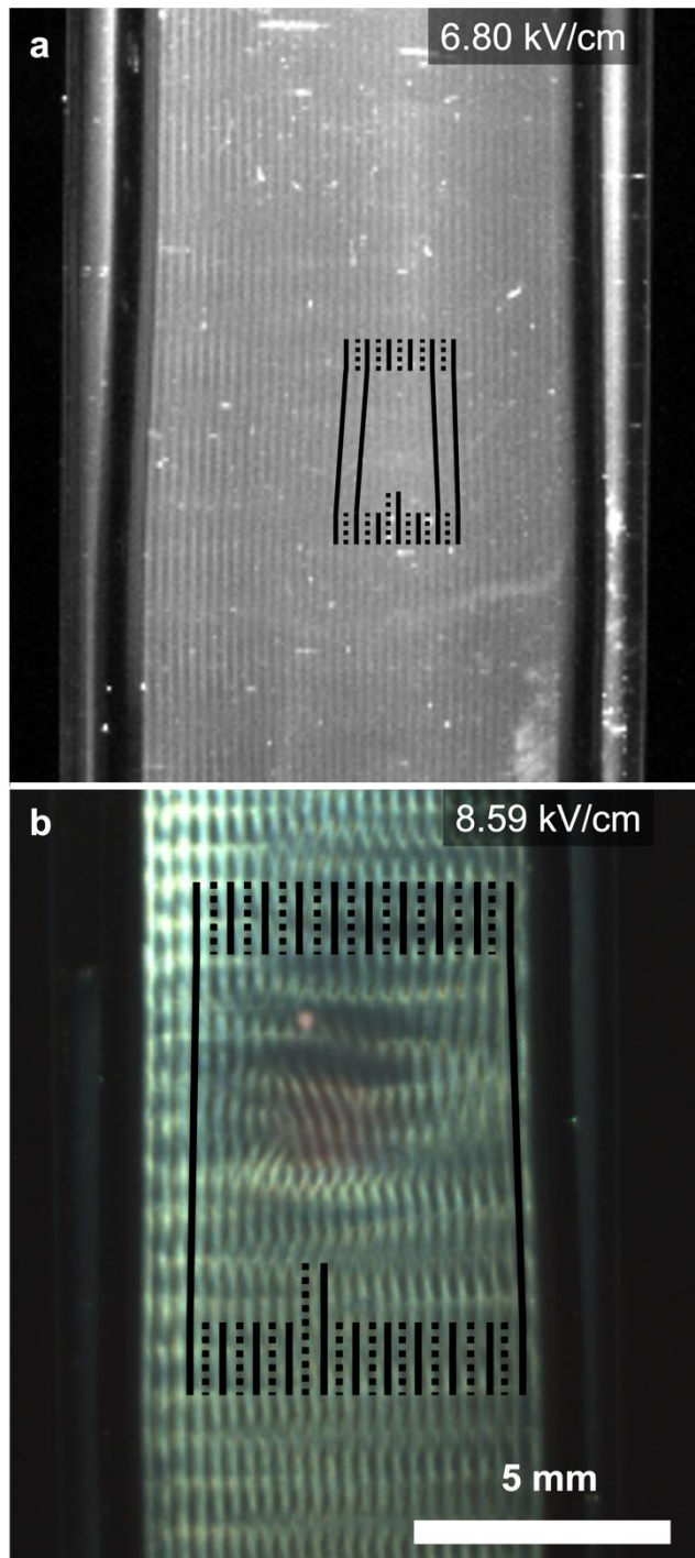
Figure 5. Observation of defects in the periodic patterns, using the experimental setup ES2. The defects always admit a pair of bright lines (two bright and two dark). a) snapshot from Supplementary Information, video S1 (monochrome camera, 1.875 fps, frame #1022) of a defect in the simple roll geometry. b) photograph of a defect where the pattern couples between x and y periodicities. The full and dotted lines are guide to the eye to distinguish the insertion of a pair of vertical bright lines.
