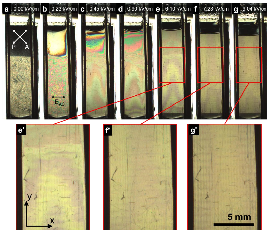
Figure 3. Observation of the sample between cross-polarizers. a) observation of the sample left overnight at rest (the sample was exposed to various electric field sequences the day before). b-g) observation under increasing electric fields. These images were recorded within a window of 4 hours from the beginning of the experiment. e'-g') insets with magnified views. The electrodes are visible as the two black vertical wires on each side of the capillary.
