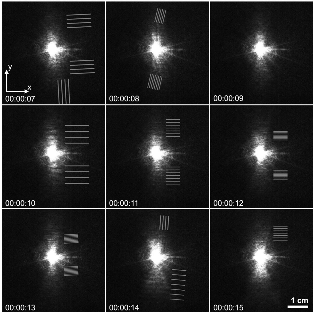
Figure 7. Snapshots from Supplementary Information, video S2 , showing laser diffraction patterns taken using the experimental setup ES4, as the field is varied from 4.3. kV/cm to 6.07 kV/cm. The distance from sample to screen was z_s = 31 cm and the scale bar indicates the distances on the screen (e.g., 0.1 cm corresponds to q \approx 0.032 \mu\text{m}^{-1} , or 2\pi/q \approx 195 \mu\text{m} ). The grey stripes are guide to the eye to distinguish the periodicities of the stripes.
