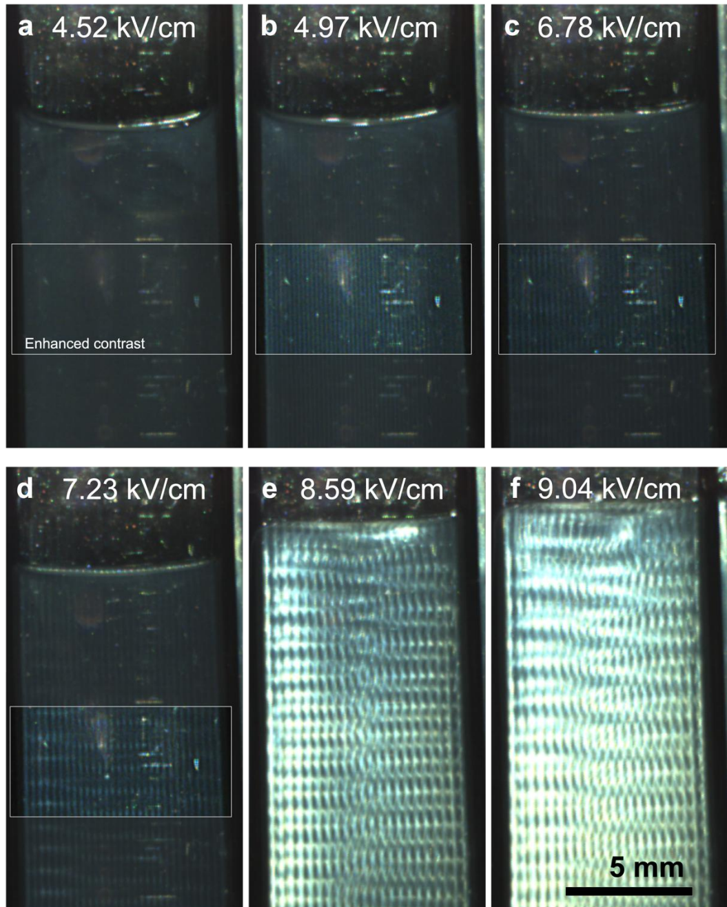
Figure 4. Observation of the sample under asymmetrical oblique illumination in transmission, using the experimental setup ES2, so the illumination is in the (y, z) plane. a) no visible pattern. b) a simple pattern of vertical periodic stripes appears, made more visible in the box with enhanced contrast. c-d) a second modulation in y appears gradually. e-f) the pattern evolves towards doubling the periodicity in y and becomes much brighter, with some coupling between the x and the y periodicities, with tilted structures.
