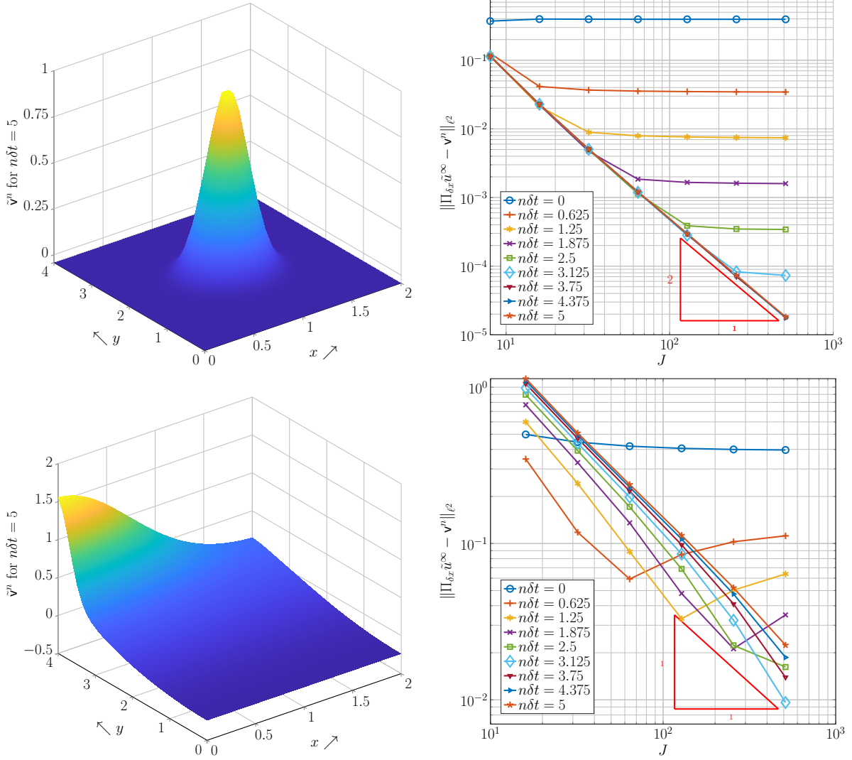
Figure 4: On the left panels, numerical solution \tilde{v}^n obtained at n\delta t = 5 and J = 32 . On the right panels, numerical error \|\Pi_{\delta x} \tilde{u}^\infty - \tilde{v}^n\| as a function of J for several values of n\delta t . On the top panels : (\alpha, x_0, y_0) = (15, 1, 2) so that the derivatives of the solution on the boundary are negligible. On the bottom panels : (\alpha, x_0, y_0) = (1, 0, 4) so that the derivatives of the solution on the boundary are not negligible.
