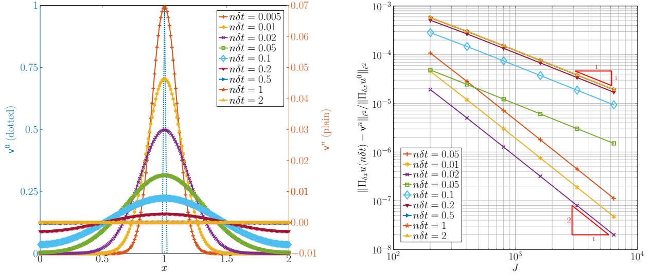
Figure 2: Numerical simulation of the solution of the homogeneous linear heat equation (1) associated to the initial datum (56) using the scheme (12) under the CFL condition (13) for several values of n\delta t . Left : Numerical approximation v^n of the solution u(n\delta t) as a function of j\delta x computed for several values of n\delta t with J = 201 (multiple scales). Right : Numerical error as a function of J for the same values of n\delta t (logarithmic scales).
