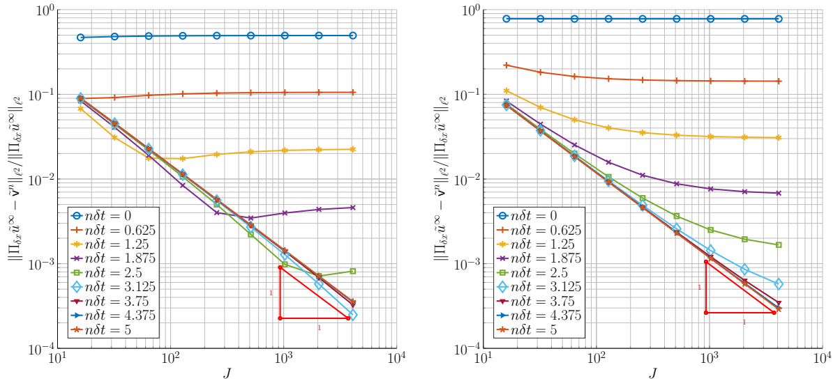
Figure 3: Numerical error as a function of J for several values of n\delta t when approximating the solution of the linear nonhomogeneous stationary heat equation (34) using the scheme (37) under the CFL condition (13) (logarithmic scales). Initial datum : \tilde{u}^0 = \langle \tilde{u}^\infty \rangle \mathbb{1} + w (left panel) and \tilde{u}^0 = \langle \tilde{u}^\infty \rangle \mathbb{1} (right panel).
