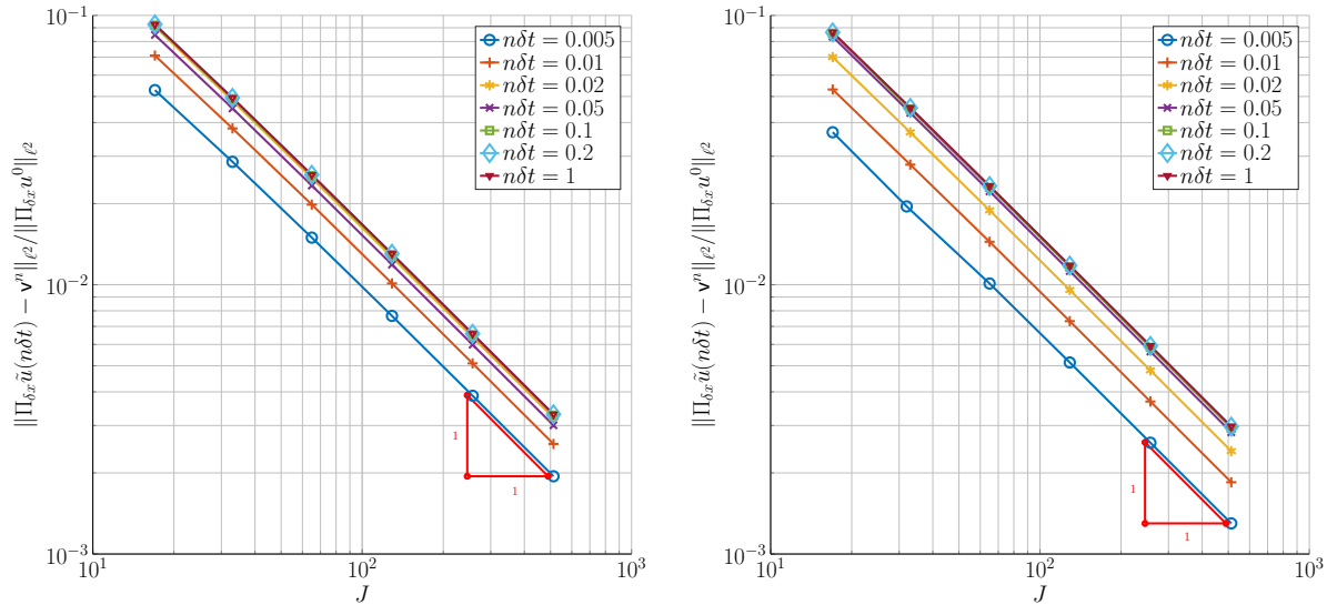
Figure 1: Numerical error as a function of J for several values of n\delta t when approximating the solution of the homogeneous linear heat equation (1) using the scheme (12) under the CFL condition (13) (logarithmic scales). The initial datum given in the text : trigonometric polynomial (left panel) and function (55) (right panel).
