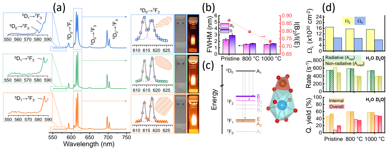
Figure 2. (a) Emission spectra ( \lambda_{\text{exc}} = 280 \text{ nm} ) of pristine (blue, top) and annealed (800 °C, green, middle; 1000 °C, orange, bottom) \text{Y}_{0.95}\text{Eu}_{0.05}\text{VO}_4 nanoparticles as 50 \mu\text{mol L}^{-1} aqueous suspensions (concentration in vanadate ions). Excitation spectra are shown in Figure S10. Insets at the left represent amplifications of the region between 550 and 590 nm, indicating the {}^5D_1 \rightarrow {}^7F_3
