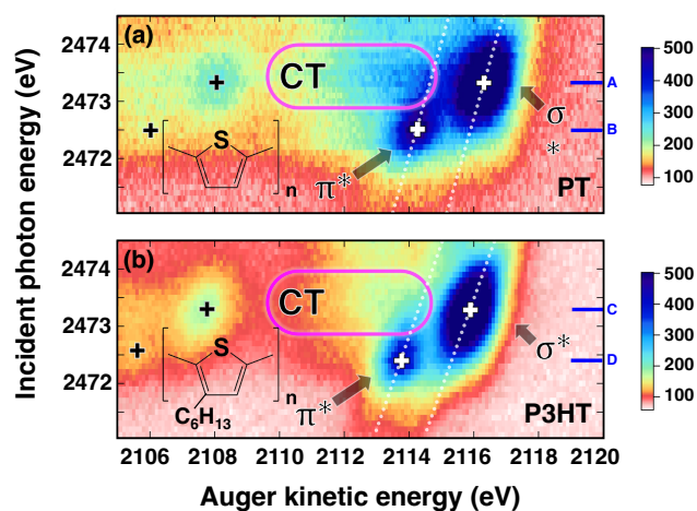
Fig. 3 2D maps of S KL_{2,3}L_{2,3} Auger spectra recorded in PT powder (a) and P3HT thin film (b). Transitions to the 2p^{-2}(1S)\pi_{S-C}^* and 2p^{-2}(1S)\sigma_{S-C}^* final states are indicated with black crosses. Transitions to the 2p^{-2}(1D)\pi_{C-C}^* and 2p^{-2}(1D)\sigma_{S-C}^* states, indicated with white crosses, are labelled as \pi^* and \sigma^* . Blue lines and adjacent labels (A-D), indicate the corresponding resonant photon energies. Diagonal dotted lines show dispersive behaviour of resonant structures. Purple stadium shapes indicate the region where the CT feature is most prominent. The maps are normalised to the background. The colour-coded intensities are on a logarithmic scale.
