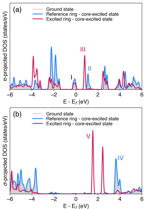
Fig. 6 DOS computed for P3HT projected on the carbon and sulfur/chlorine atoms of the excited and reference rings, and on the angular momentum components (a) p_y ( \pi -orbital character) and (b) s+p_x+p_z ( \sigma -orbital character). The energy of states is shown relative to the Fermi level. At the reference ring, the projected DOS in the ground state (grey area) and in a core-excited state (blue line) are nearly identical. The roman numerals label the occupied \pi band (I), the first unoccupied \pi^* band (II) and the unoccupied \sigma^* band (IV). At the excited ring, the projected DOS in a core-excited state (red) contains the split-out \pi^* MO (III) and the split-out \sigma^* MO (V).
