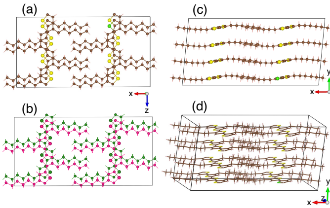
Fig. 2 Ball and stick illustration of the employed P3HT simulation cell: (a-b) bottom, (c) side, and (d) diagonal views. The XZ plane is parallel to the sample surface. Colour code: brown for carbon, yellow for sulfur, green for chlorine (Z+1 approximation), light pink for hydrogen. In panel (b), different polymer layers are depicted in pink and green to show the lateral displacement between the chains when stacked. All the structures' rendering were generated using the VESTA 32 software.
