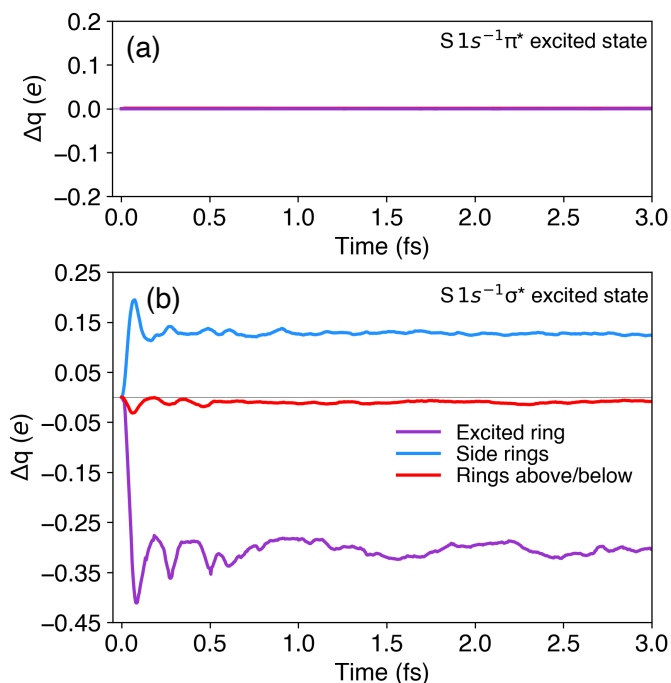
Fig. 9 Bader charge analysis of the selected rings in P3HT for the first 3 fs of propagation in the core-excited states (a) 1s^{-1}\pi^* and (b) 1s^{-1}\sigma^* . The grey line denotes \Delta q=0 . Negative (positive) values indicate electron depletion (accumulation).
