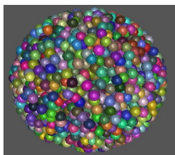
Figure 1: Spheroid generated by CPOP
