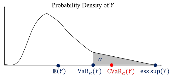
Fig. 1. The Conditional Value-at-Risk (CVaR) quantifies the upper tail of a cost distribution. For an absolutely continuous, bounded random variable Y representing a cost and \alpha \in (0, 1] , we illustrate the expected cost in the \alpha \cdot 100\% worst cases, which is CVaR_\alpha(Y) in this setting. The area of the shaded region is \alpha . The expectation of Y , the Value-at-Risk of Y at level \alpha (the lowest cost in the \alpha \cdot 100\% worst cases), and the essential supremum of Y are also shown.
