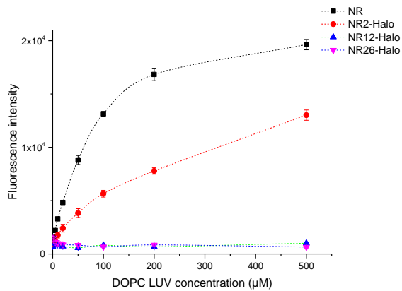
Figure 3. Titration of studied NR derivatives in PB 20 mM at pH 7.4 with DOPC LUVs. Excitation wavelength 540 nm, emission wavelength 640 nm. The indicated concentration corresponds to the lipid concentration.
