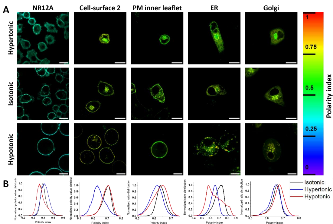
Figure 8. (A) Polarity imaging of transfected KB cells expressing HaloTagged proteins at various localization in CLSM under condition of osmotic stress. NR12-Halo at 1 \mu\text{M} in Opti-MEM was used as fluorescent probe. Scale bars: 20 \mu\text{m} . (B) Distribution curves of the polarity index normalized at their maximum.
