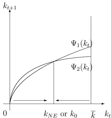
Figure 6: Dynamics when \beta_2 = 0 or \beta_2 low enough
