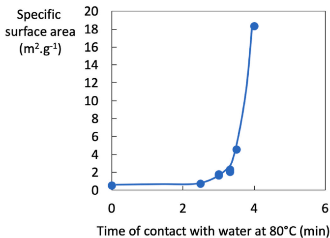
Fig. 4. Specific surface area of powders activated for different times in water at 80 °C (concentration of AlSi12 powder in water = 400 g.L -1 ).
