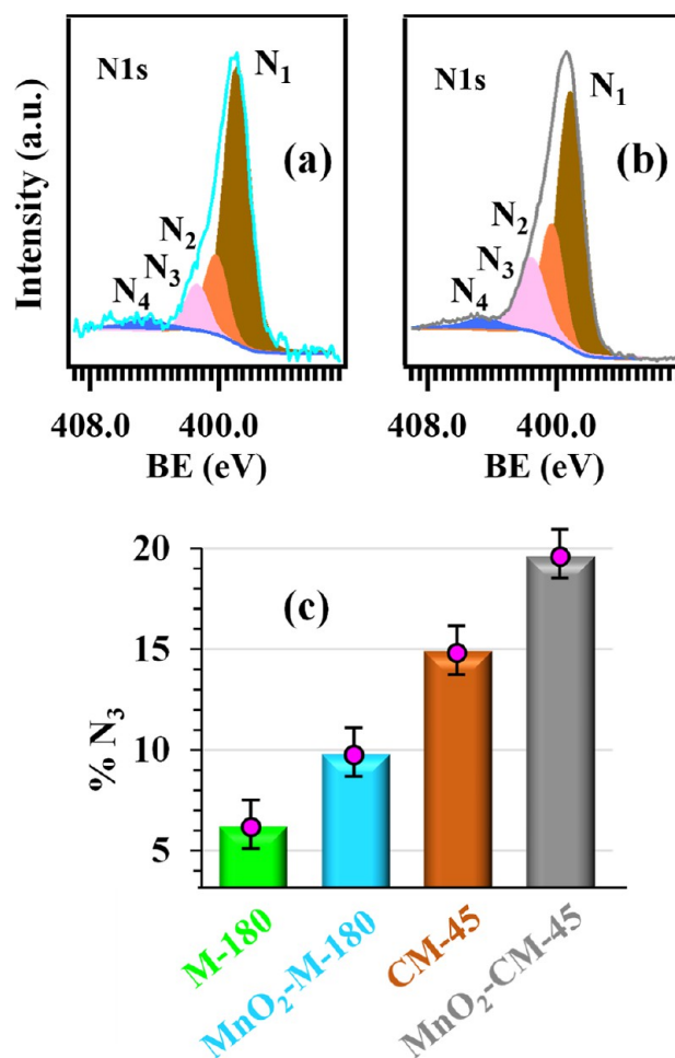
Figure 7. N 1s photopeaks for representative \text{MnO}_2 + \text{g-CN} samples: (a) \text{MnO}_2\text{-M-180} ; (b) \text{MnO}_2\text{-CM-45} . Color codes for the different fitting components identifying nonequivalent nitrogen atoms are defined in Figure 6c. (c) Percentage contribution of the \text{N}_3 component to the overall N 1s signal for the analyzed specimens.
