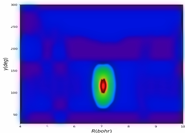
Fig. 8 Wavefunction cut ( R, \gamma ) of \text{H}_2\text{O-HCN} at E= 224.841 \text{ cm}^{-1}
