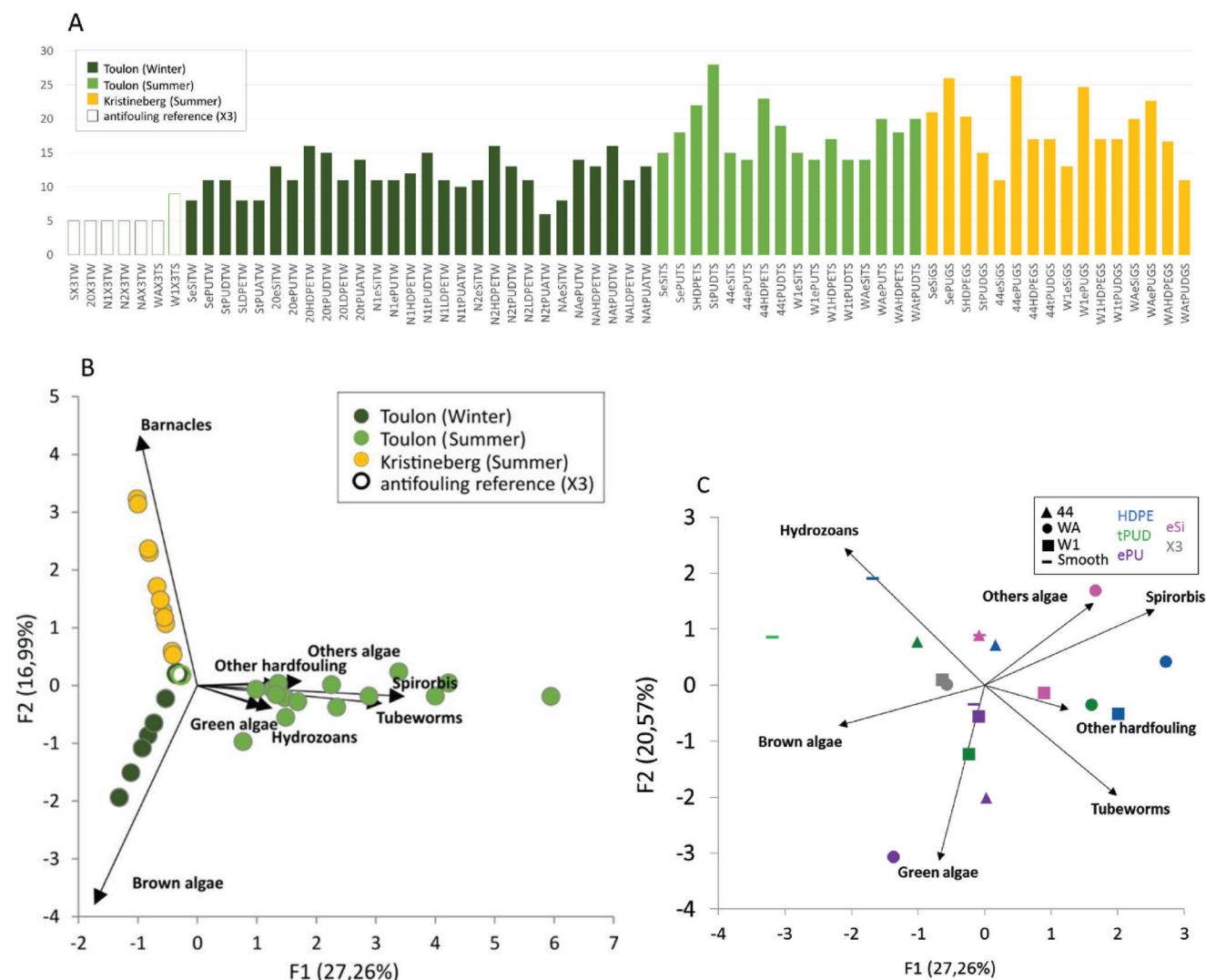
Figure 7. A) Efficacy parameter of each substrate and B) Principal Component Analysis (PCA), based on the percentage of coverage of the main groups of macrofouling visually observed in Kristineberg Center and Toulon, with C) a focus on the summer season at Toulon.
