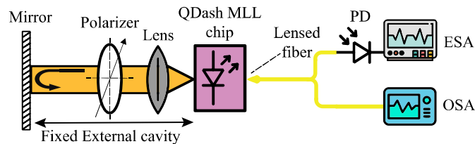
Fig. 1. Experimental setup. QDash MLL: Quantum-Dash Mode-Locked Laser, PD: Photodiode, ESA: Electrical Spectrum Analyzer, OSA: Optical Spectrum Analyzer.
