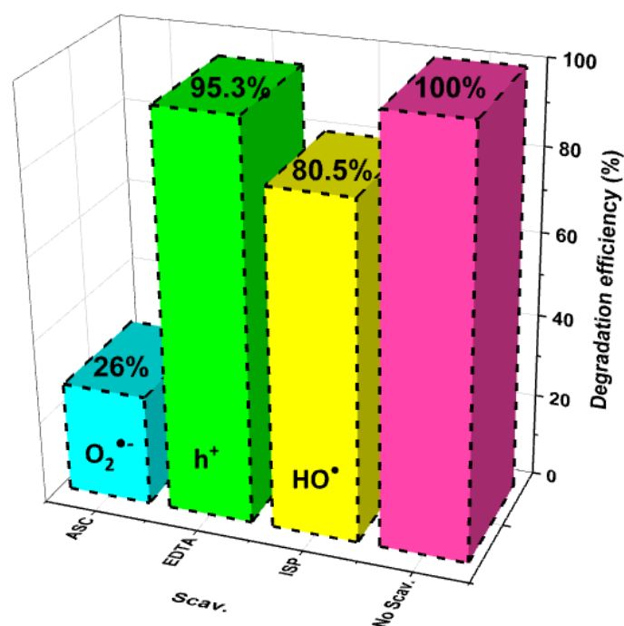
Figure 14. The actives species trapping experiments for degradation efficiency of RhB dye by BiOBr@Kaol
