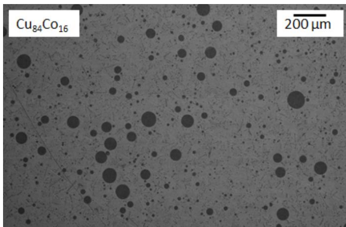
Fig. 14 Dispersion of Co-rich L1-droplets in the Cu-rich matrix L2. The alloy has been undercooled and solidified during parabolic flight in low gravity.
