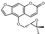
(-)-Oxypeucedanin
