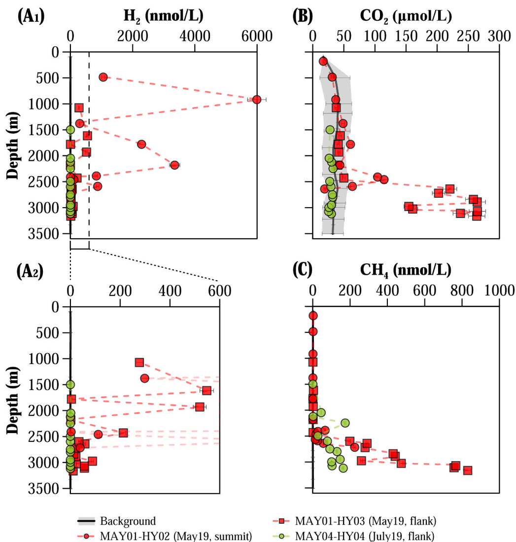
Fig. 4. Depth profiles of studied dissolved gases at the eruption site during the May 2019 eruption (in orange) and two months later (in green). MAY01-HY02 cast (from May 2019) was performed at the volcano summit while MAY01-HY03 (from May 2019) and MAY04-HY04 (from July 2019) were sampled at the northern flank of the volcano. (A 1 ) H 2 profiles; (A 2 ) Zoom in H 2 profiles for H 2 concentrations from 0 to 600 nmol/L; (B) CO 2 profiles; (C) CH 4 profiles. Evaluated background is represented by the bold line and the grey envelop. (For interpretation of the references to colour in this figure legend, the reader is referred to the web version of this article.)
