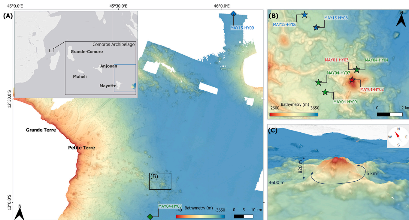
Fig. 1. (A) Map of the site with reference CTD casts and 50 m-resolution bathymetry using WGS 84 geodetic system (Geo-Ocean (Ifremer), 2022), (B) Bathymetry (30 m-resolution) of the volcano edifice with CTD casts performed above the volcano and above lava flows, (C) 3D representation of the volcano edifice (vertical exaggeration x2).
