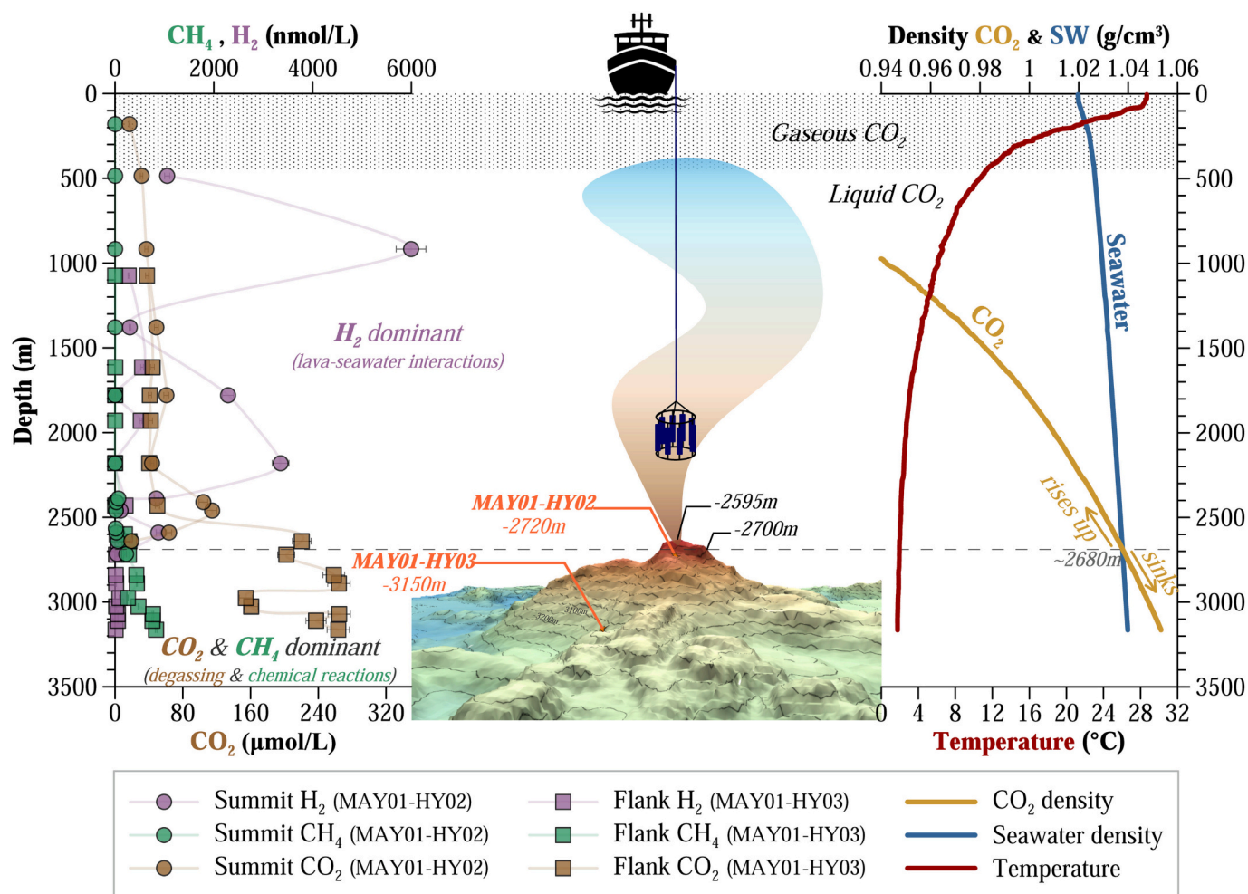
Fig. 9. Composite representation of gas concentration profiles, water column physical parameters and bathymetry of the Fani Maoré Seamount during the May 2019 eruption (MAYOBS1 cruise). Profiles of H 2 , CO 2 and CH 4 were measured at the summit and above the northern flank of the volcano. Pure-CO 2 density changes with the water column depth at the volcano was calculated using Span and Wagner's equation of state (Span and Wagner, 1996). Standard-seawater density profile was calculated from CTD data recorded at both sites and Archer's thermodynamic model for NaCl (Archer, 1992). Temperature profile was extracted from CTD data recorded at both sites. 3D representation of the volcano edifice was made using 30 m-resolution bathymetry (vertical exaggeration x2), with counter lines at 50 m intervals (Geo-Ocean (Ifremer), 2022).
