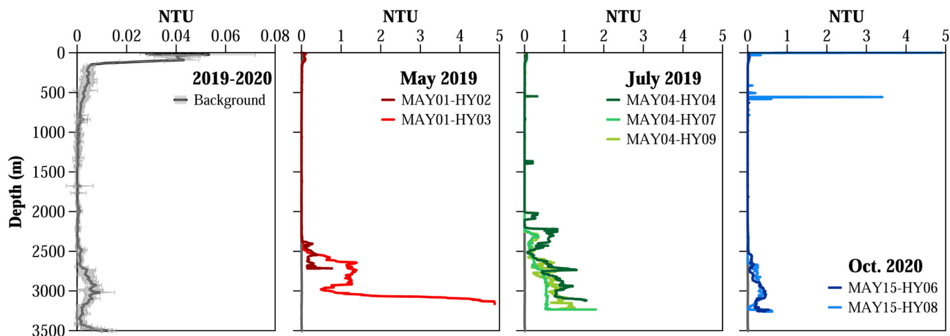
Fig. 2. Turbidity profiles determined by background evaluation, and measured for the studied hydrocasts from May 2019, July 2019 and October 2020 (MAYOBS1, MAYOBS4 and MAYOBS15 cruises, respectively). Please pay attention to the differences in NTU scales between the background profile and the others.
