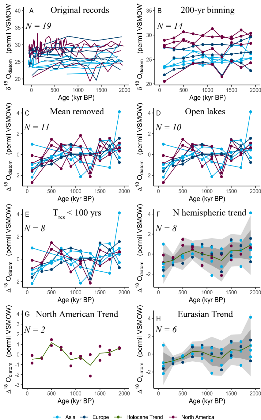
Figure 5. Common Era Northern hemispheric records (45-90°N) compiled in this study. A) Original records, B) data binned to 200 year intervals, only showing records covering at least 7 bins, C) binned records with mean of individual records removed, D) filtered for records from open lakes only, E) filtered for records from lakes with t_{\text{res}} < 100 yrs, F) NH trend, calculated as mean of all records in each bin. Shadings show 1 and 2 standard deviations, respectively. G) North American and H) Eurasian trend.
