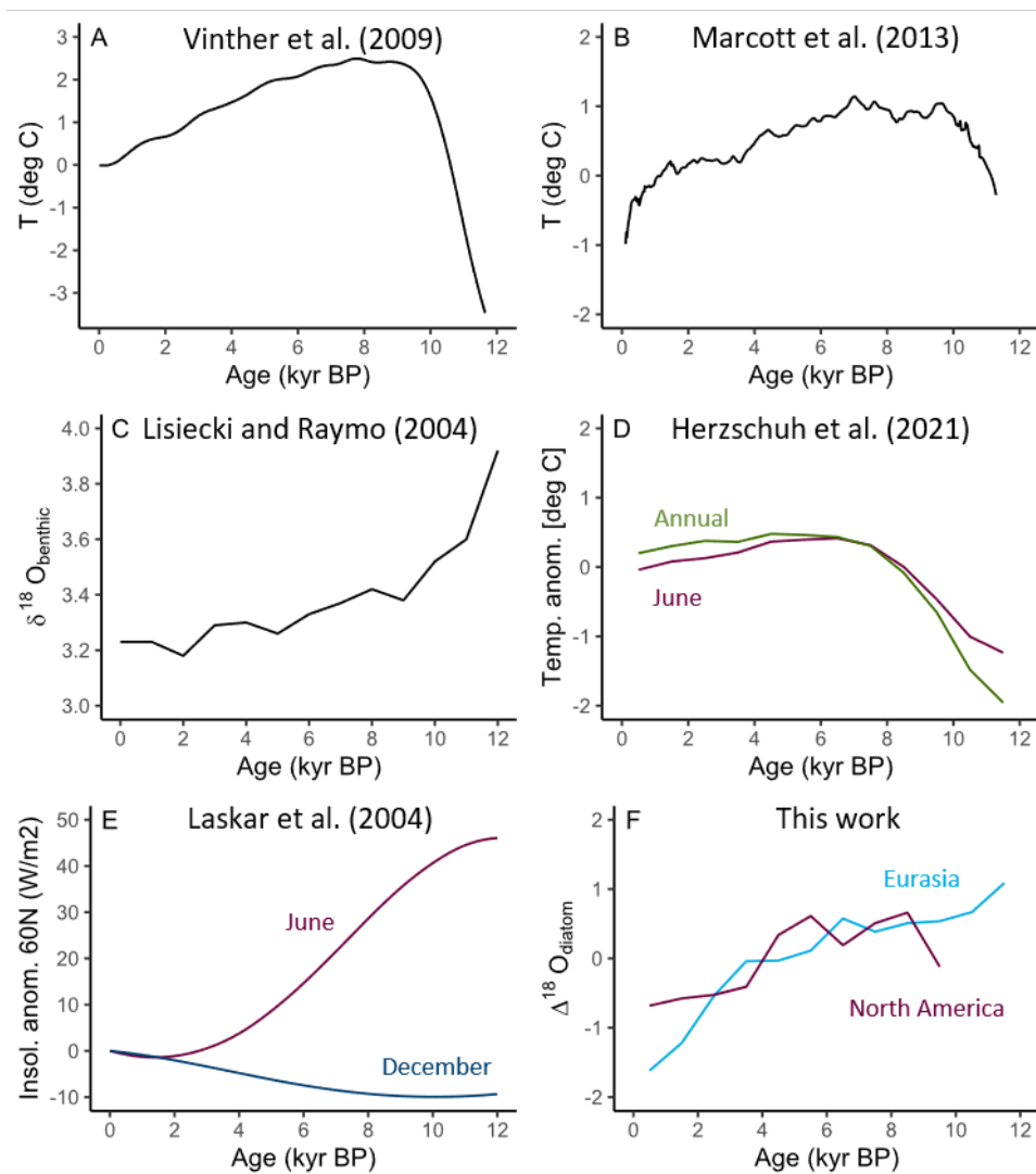
Figure 8. Combined Trend of \delta^{18}\text{OBSi} compared to other climate reconstructions. A) Greenland ice sheet temperature reconstruction, B) Multi-proxy temperature reconstruction (30-90 N), C) global stack of \delta^{18}\text{O} from benthic foraminifera, D) temperature reconstruction (45-90 N) based on pollen data, E) Insolation anomaly for June and December, F) Combined Eurasian and North American Trend from \delta^{18}\text{OBSi} records (this work).
