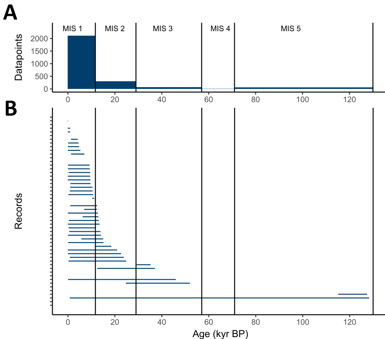
320 Figure 2. Temporal coverage by records and datapoints during MIS 1 – MIS 5. a) Total number of datapoints available 325 during each Marine Isotope Stage. b) Temporal coverage of records.
