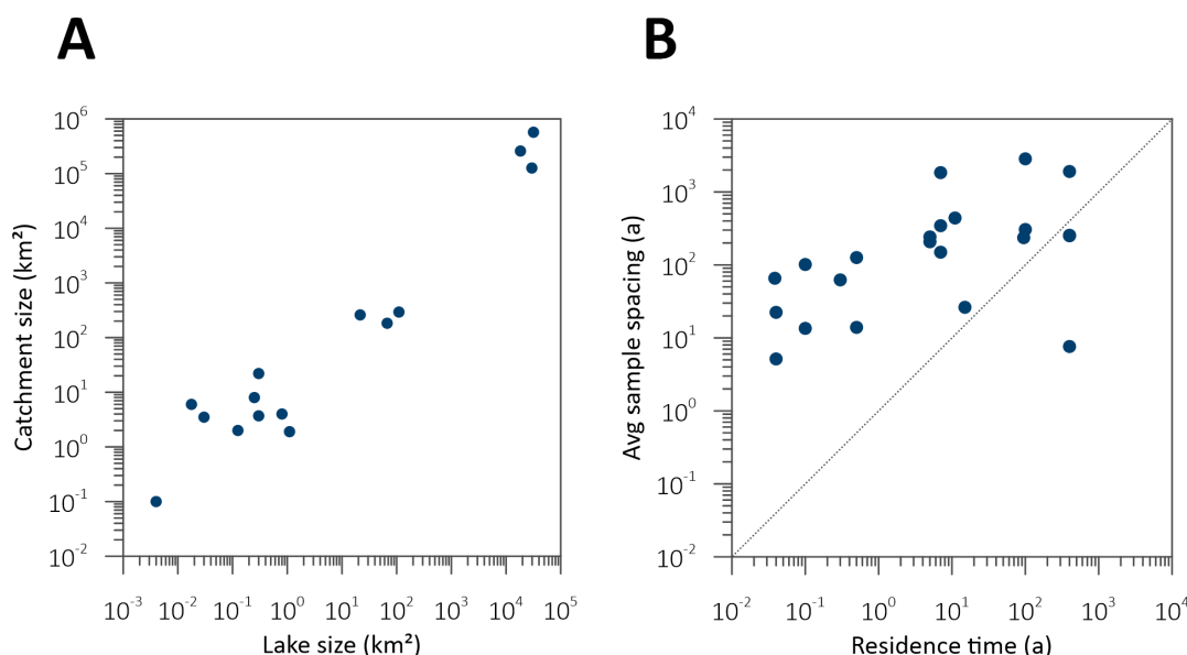
Figure 4. A) Depiction of corresponding lake and catchment sizes of the records compiled within this study. One lake may correspond to more than one records. Note that records from Paleo-lakes and lakes with incomplete information on lake and catchment size were not considered for this figure ( N=33 ). B) Depiction of corresponding sampling intervals and t_{\text{res}} . Note that records from lakes without information on t_{\text{res}} were not considered for this figure ( N=37 ).
