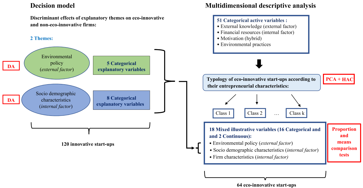
Fig. 1. Methodology overview.
