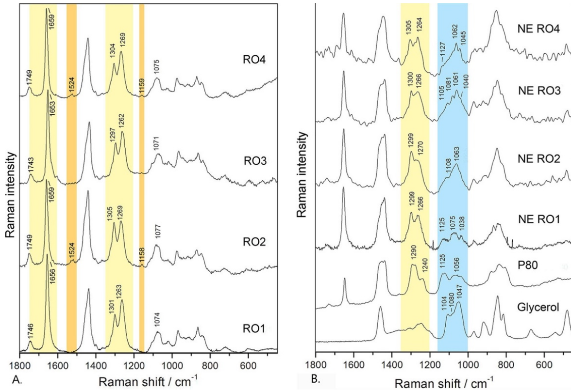
Figure 9: Raman spectra of NEs. A) Raman spectra of different red raspberry oils (ROs): RO1—cold pressed refined, non-organic oil; RO2—cold-pressed, unrefined, organic oil; RO3—CO 2 extracted unrefined, non-organic oil; RO4—CO 2 extracted, unrefined, organic oil. B) Raman spectra emulsified oils as nano-emulsions. Adapted with permission from [91], see details in the text.
