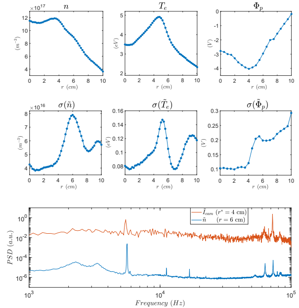
FIG. 2. Radial profiles of the density, electron temperature, and plasma potential mean values (top row) and fluctuations (middle row) at p_0 = 1 mTorr. Plasma parameters measurements were made with 5-tips ( n , T_e ) and emissive ( \Phi_p ) probes. Bottom: Power Spectral density of the plasma density and light intensity fluctuations (computed from the average value of a 5 \times 5 pixel box on the images).
