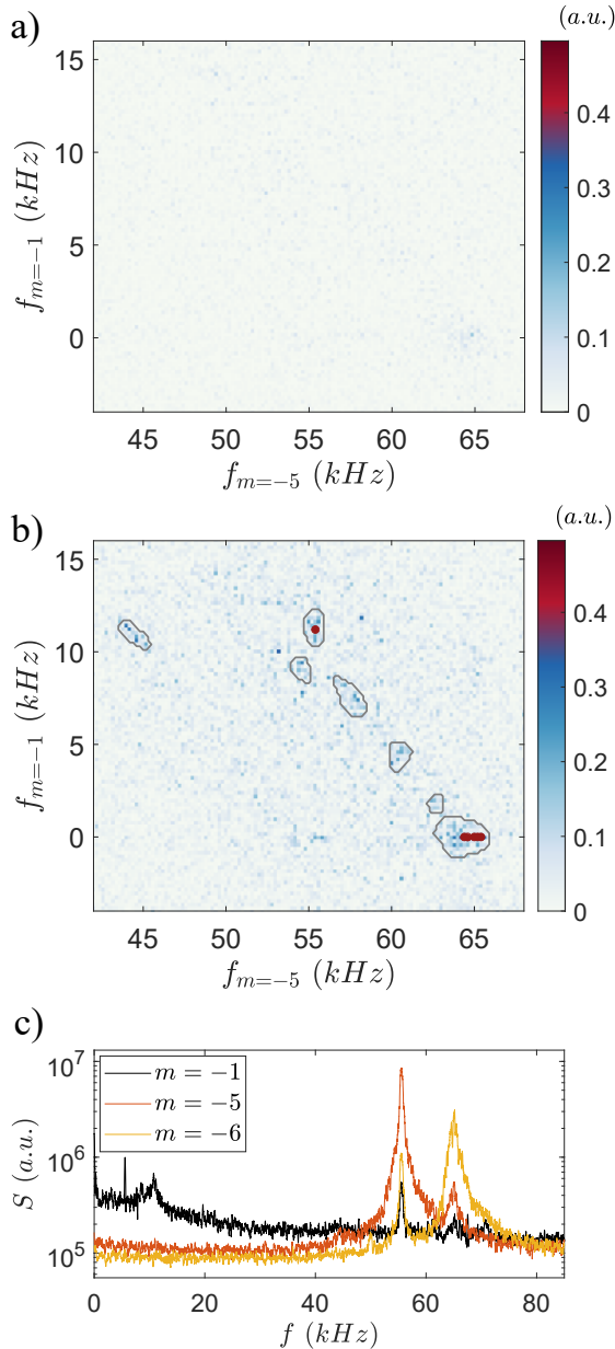
FIG. 11. Maps of the threshold b_0^2 (a) and bicoherence b^2 (b), corresponding to the three-wave interaction (m = -5) + (m = -1) \leftrightarrow (m = -6) . (c) Frequency power spectra of modes m = -1 , m = -5 and m = -6 from 2D-FT computed at r^* = 3.3 cm. B = 170 G and p_0 = 1.3 mTorr.
