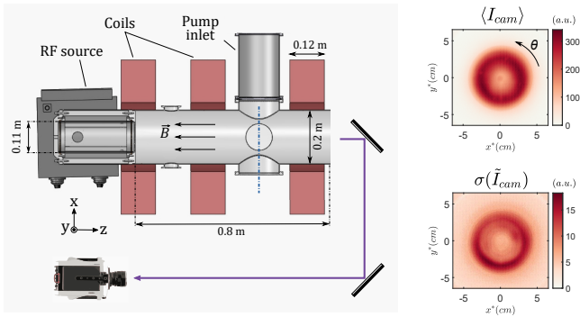
FIG. 1. Left: sketch of the experimental set-up. The dashed blue line indicates where probe profiles are measured. Right: mean image of the light intensity collected by the camera (up), and standard deviation of the fluctuations around this average value (bottom), for p_0 = 1 mTorr.
