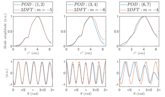
FIG. 7. Comparison of (top) radial and (bottom) azimuthal profiles of the POD and 2D-FT modes, at p_0 = 1.3 mTorr, for the (left) m = -5 , (center) m = -6 and (right) m = -4 modes.
