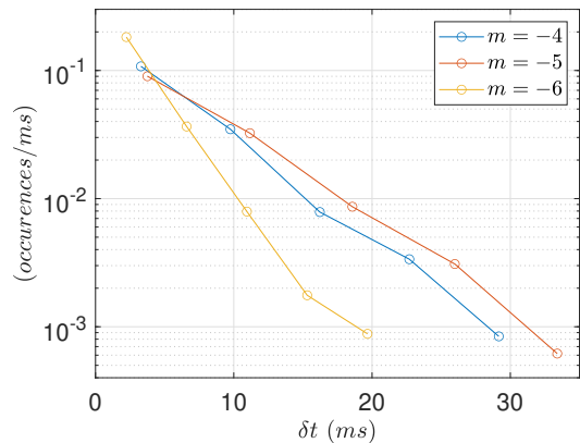
FIG. 10. Residence time PDF, obtained for a neutral pressure p_0 = 1.30 mTorr.
