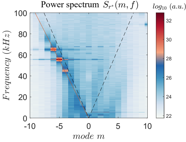
FIG. 4. Power spectrum of the raw light intensity fluctuations from camera imaging, taken on a corona of radius r^* = 3.3 cm for p_0 = 1.3 mTorr. Dispersion relations are plotted from experimental fits of the power spectrum maxima (red) and from the ion acoustic speed (black) (see section IV).
