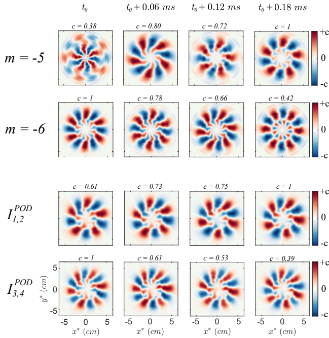
FIG. 6. Evolution of 2D-FT modes m = -5 , m = -6 and POD reconstructed modes I_{1,2}^{POD} and I_{3,4}^{POD} , during the exchange event highlighted by the dashed-black box in Fig. 5, for p_0 = 1.3 mTorr.
