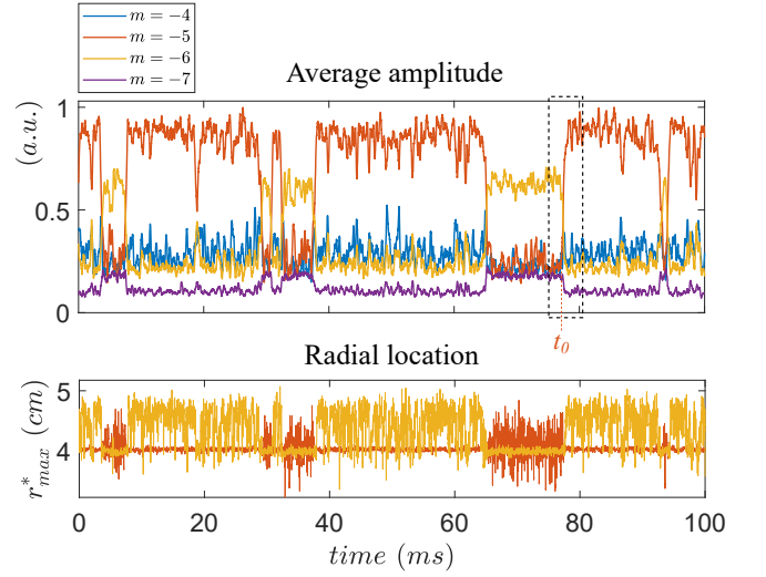
FIG. 5. Time evolution of m -mode average amplitudes extracted by 2D-FT, for p_0 = 1.3 mTorr.
