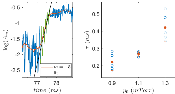
FIG. 9. Left: time evolution of m -modes average amplitudes, extracted by 2D-FT. Left: fit of the 2D-FT m = -5 mode growth rate at an exchange event with m = -6 mode, for p_0 = 1.3 mTorr. The fit is done on a selected interval of the raw data (light blue). The red curve is the result of a filter. Right: Evolution of the growth time scale of m = -5 mode, evaluated during exchange events, as a function of the pressure p_0 .
