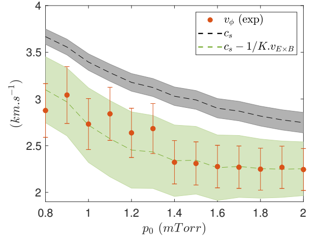
FIG. 8. Comparison between the experimental phase velocity (red dots), the ion sound velocity c_s (black curve), and its Doppler shifted values (green curve).
