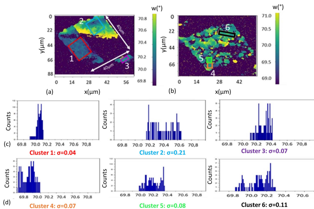
Figure 5 (a) A COM map for \omega of GaN structure 1 with p = 0.5 \mu\text{m} . (b) A COM map for \omega of GaN structure 2 with p = 1 \mu\text{m} . (c) Three histograms showing the distribution of \omega in clusters 1, 2 and 3 inside structure 1. (d) Three histograms showing the distribution of \omega along clusters 4, 5 and 6 inside structure 2 (the binning step corresponds to 0.1^\circ ).
