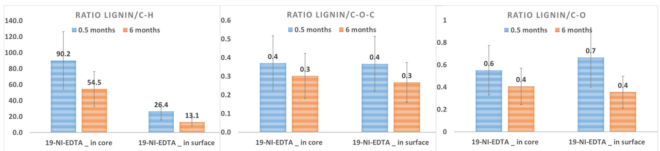
Figure 7. Ratios of lignin and carbohydrates for impregnated and non-impregnated samples subsequently treated with EDTA. FTIR analysis, carried out after an immersion period of 0.5 months and 6 months.
