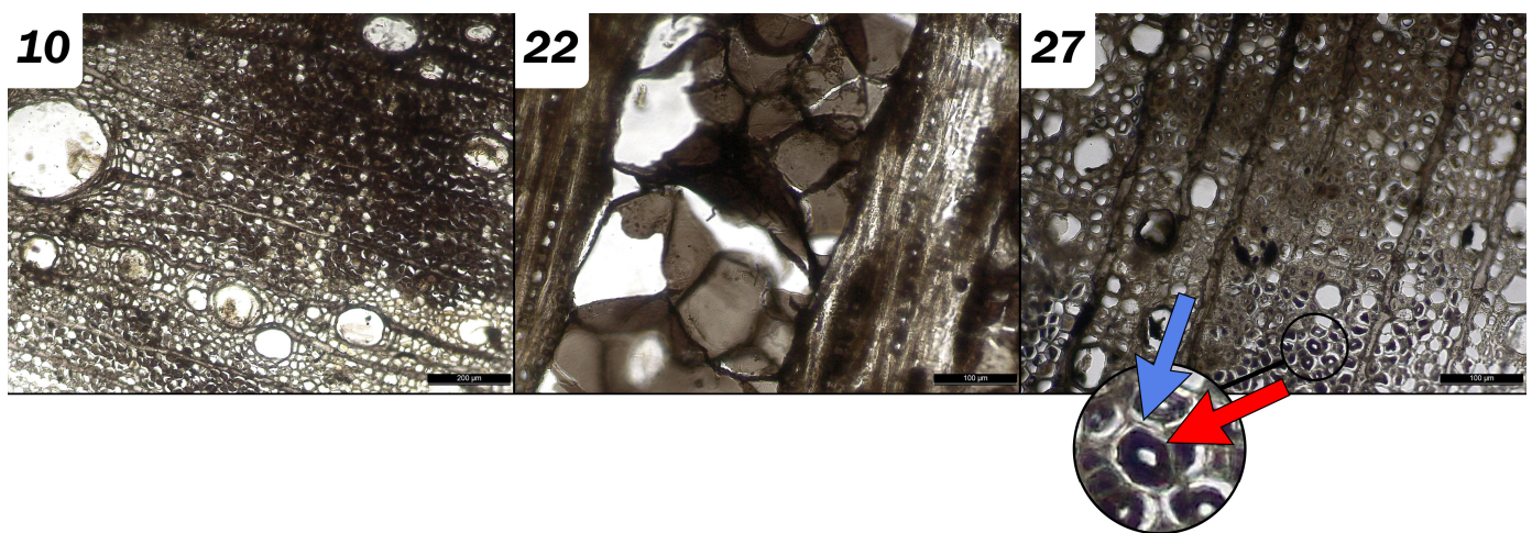
Figure 4. Sections of archaeological samples after treatment. #10—DTPA cross section showing the decayed secondary wall impregnated with black iron compounds. Scale bar: 200 \mu\text{m} ; #22—Sodium dithionite + DTPA, longitudinal tangential section showing blackish tyloses in a vessel lumen; #27—Sodium dithionite + DTPA, cross section: the red arrow points to the decayed secondary wall impregnated with black iron compounds, while the blue arrow points to the remaining compound middle lamella. Scale bar: 100 \mu\text{m} .
