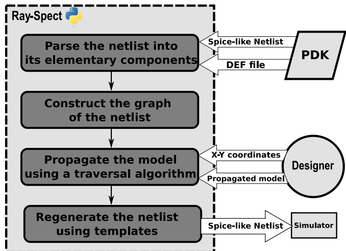
Fig. 4: Overview of the simulation flow using Ray-Spect
