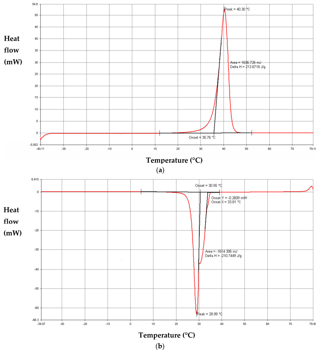
Figure 14. Analysis of thermograms of RT35HC during (a) heating and (b) cooling at 10\text{ }^{\circ}\text{C}\cdot\text{min}^{-1} .
