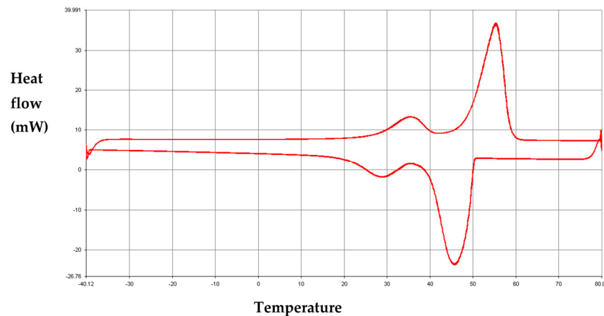
Figure 19. DSC thermograms of RT50 under ten thermal cycles at 10 °C.min -1 .
