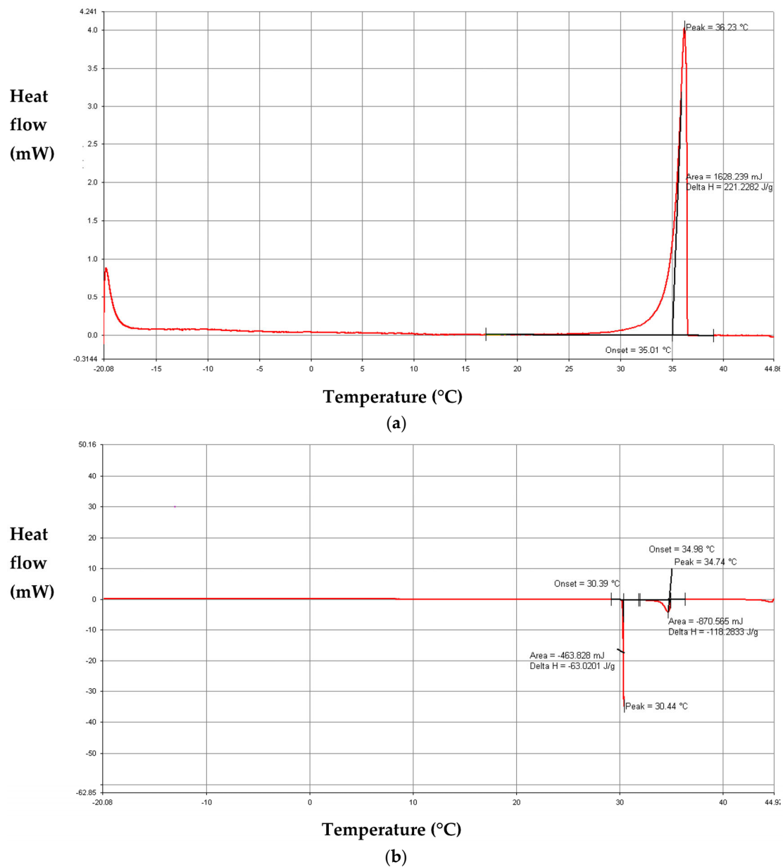
Figure 15. Analysis of thermograms of RT35HC during (a) heating and (b) cooling at 0.2\text{ °C}\cdot\text{min}^{-1} .
