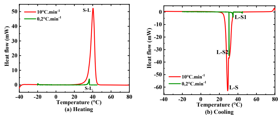
Figure 13. DSC results of RT35HC with heating–cooling rates of 10 °C.min -1 and 0.2 °C. min -1 .
