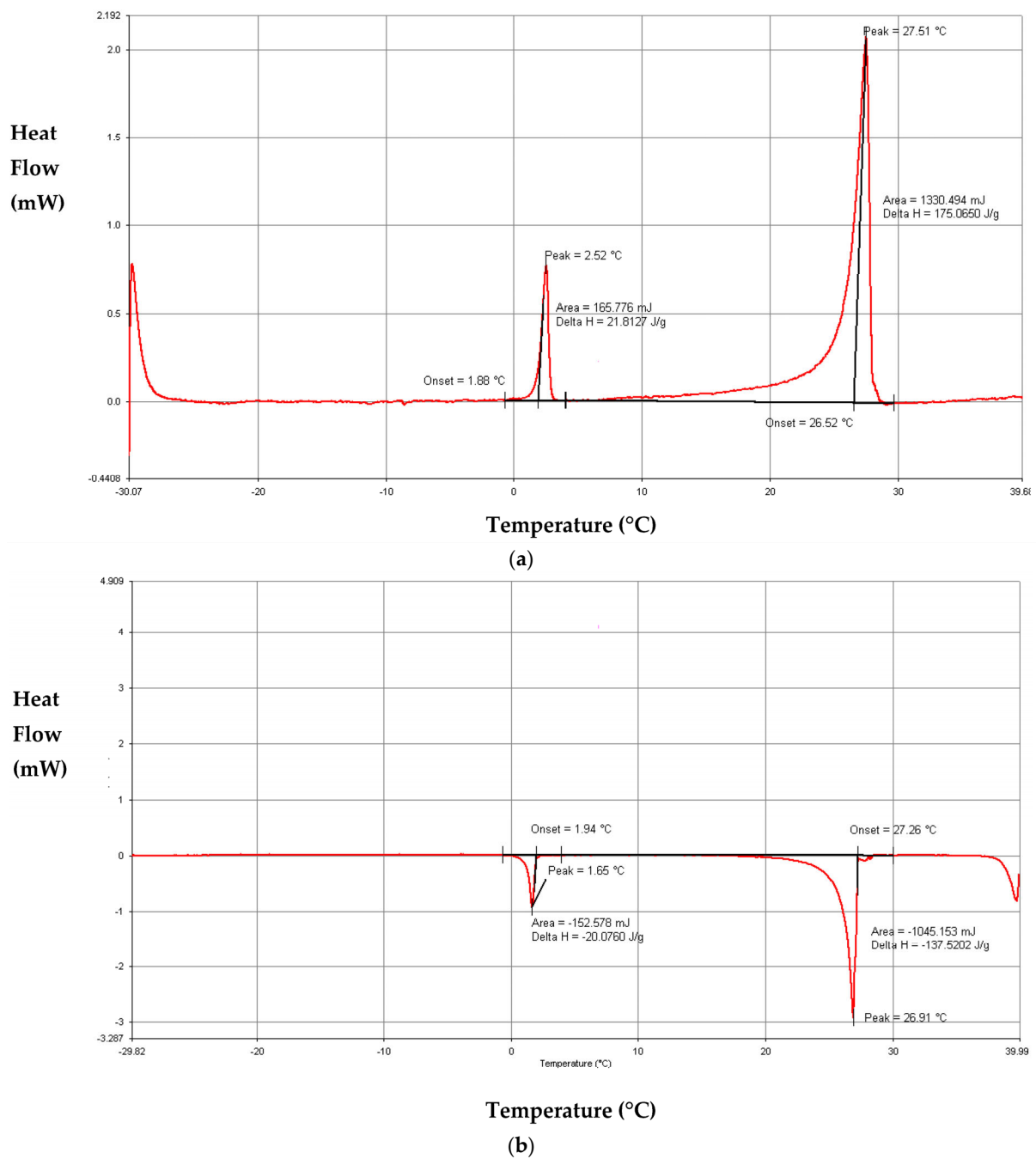
Figure A2. Analysis of thermograms of RT27 during (a) heating and (b) cooling at 0.2\text{ }^{\circ}\text{C}\cdot\text{min}^{-1} .
