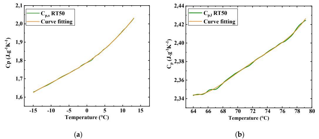
Figure 25. Evolution of the specific heat of RT50 in (a) the solid state and (b) the liquid state with temperature.
