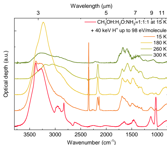
Fig. 1. MIR spectra of a \text{CH}_3\text{OH}:\text{H}_2\text{O}:\text{NH}_3=1:1:1 exposed to 40 \text{ keV H}^+ and then warmed up to 300 \text{ K} with a constant heating rate of 3 \text{ K min}^{-1} .
