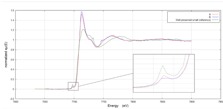
Fig. 6 XANES spectra at the Co K-edge of smalt from both cross-sections A and B and from a commercial smalt (Deffner & Johann Smalte 9001050)
