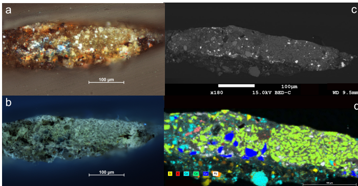
Fig. 5 a: Image of cross-section B under white light. b: Image of cross-section B under UV light. c: back scattered electron image of cross-section B. d: elemental map of cross-section B, in yellow the Si, in red the K, in cyan the Ca, in green the Co, in blue the Cu and in white the Pb.
