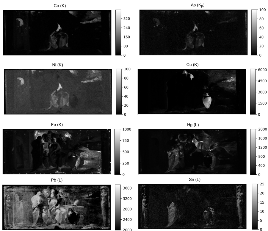
Fig. 3 Elemental distribution extracted from MA-XRF scan
