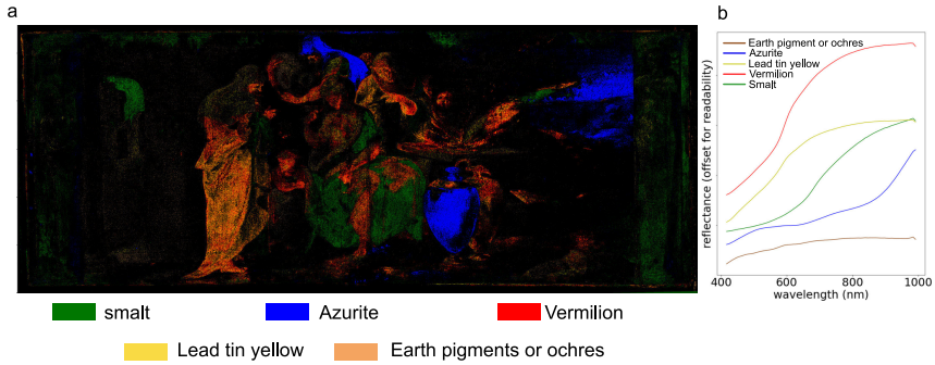
Fig. 4 Reflectance spectra and associated distribution map obtained from reflectance imaging spectroscopy (RIS). a: SAM map corresponding to reflectance spectra shown in b. b: Reflectance spectra of end-members labeled as : smalt (green color), vermilion (red color), azurite (blue color), lead tin yellow (yellow color), earth pigments or ochres (brown color).
