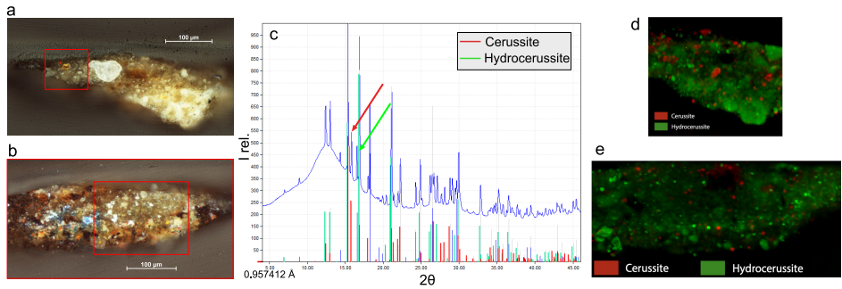
Fig. 7 a: optical image of cross-section A where area of the 2D- \mu XRD mapping is indicated. b: optical image of cross-section B where area of the XRD analysis is indicated. c: diffractogram of cross-section A, characteristic peaks of cerussite and hydrocerussite are indicated. Arrows indicate peaks used to extract maps. d: superposition of cerussite and hydrocerussite maps of the studied zone of cross-section A. e: superposition of cerussite and hydrocerussite maps of the studied zone of cross-section B
