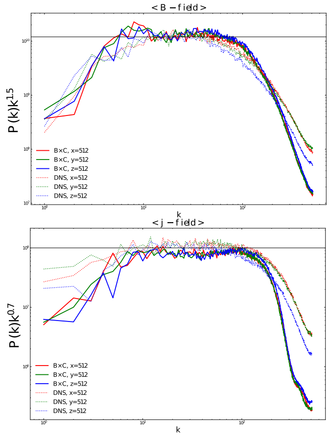
FIG. 7. Same as Fig. 6, but where the spectra have been compensated.
