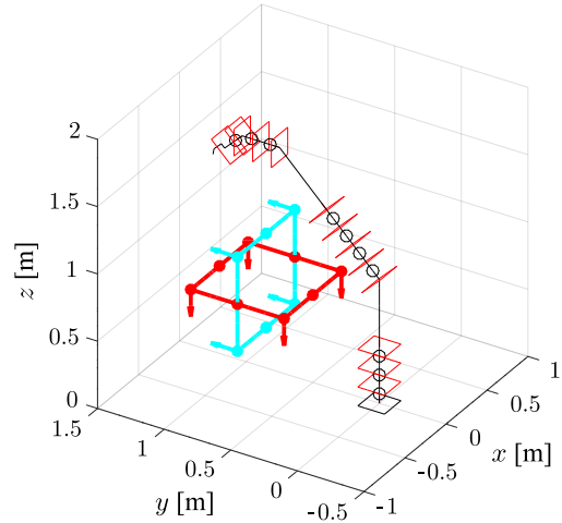
Figure 5: The two paths used to validate the designs obtained from the optimization process and a version of Nimbl'bot robot of size: l_1 = 0.5 m, l_2 = 0.5 m, \beta_1 = \pi/4 , \beta_2 = \pi/4 , \beta_3 = \pi/4 .
