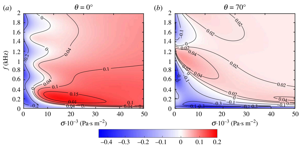
Figure 5. Influence of the static air-flow resistivity on the absorption coefficient. Difference \alpha_3 - \alpha_0 as a function of f and \sigma for (a) \theta = 0^\circ and (b) \theta = 70^\circ .
