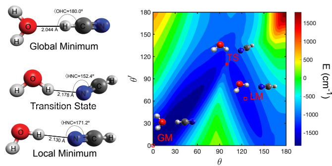
FIG. 2. Contour plot of the \text{H}_2\text{O} -HCN PES as a function of \theta and \theta' coordinates (in deg) [minimized over (R, \phi, \phi') coordinates]. The transition state (TS) indicated by red star symbol represents a barrier between the global (GM) and local (LM) minima (locations represented by red squares). The energy of the transition state is E_{TS} = -1190.5 \text{ cm}^{-1} .
