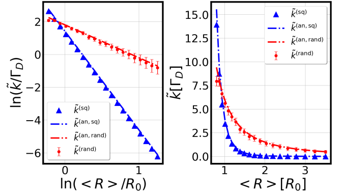
Figure 3. Left: Numerical computation of the macroscopic mean-field rate of RET \tilde{k}^{(\text{rand})} in log-scale (red points) from Eq.31, as a function of the average distance \langle R \rangle between individual excited donors and their nearest-neighbor acceptor molecules. An average is performed on 1000 configurations of disorder, for various random distributions of molecules on the square network shown in Fig. 1-Right. The error bars represent one standard deviation, illustrating the uncertainty due to fluctuations in the spatial location of molecules that varies from sample to sample. The dash-dotted red curve is obtained from the analytical rate \tilde{k}^{(\text{an,rand})} in Eq.36. The same calculation for the rate \tilde{k}^{(\text{sq})} is shown (blue triangles) for the case of one perfectly ordered square network of molecules shown in Fig. 1-Left. The dash-dotted blue curve is given by the analytical rate \tilde{k}^{(\text{an,sq})} in Eq.37. Right: Same plots but in linear scale. Parameters: N_D = N_A = N/2 = 50 , and R_c = 0.8R_0 .
