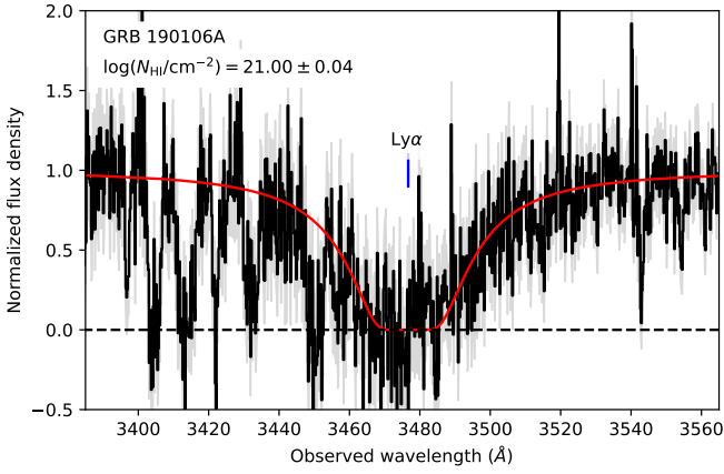
Fig. A.1. VLT/X-shooter GRB afterglow spectrum of GRB 190106A. The normalized 1D spectrum is shown in black, with the associated error spectrum shown by the gray region. The best-fit damped Lyman- \alpha profile with \log(N_{\text{HI}}/\text{cm}^{-2}) = 21.00 \pm 0.04 is shown in red.
