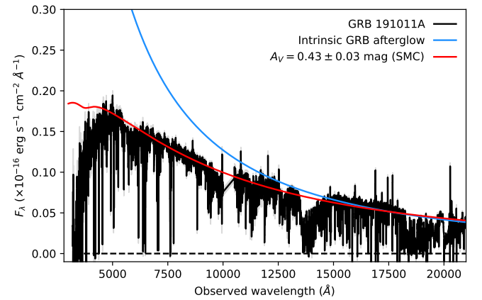
Fig. A.9. Same as Fig. A.3 but for GRB 191011A, with a best-fit of A_V = 0.43 \pm 0.03 mag.
