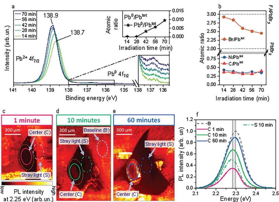
Figure 2. a) Pb 4f 7/2 spectra of pristine FAPbBr 3 : the main peak is ascribed to Pb 2+ , the smaller feature to Pb 0 (zoom in the bottom inset). The Pb 0 /Pb tot atomic ratio is shown in the top inset. b) Br/Pb tot , N/Pb tot , and C/Pb tot atomic ratios for pristine FAPbBr 3 . Dashed lines indicate the expected Br/Pb tot ratio in pristine FAPbBr 3 and PbBr 2 . c-e) PL maps at 2.25 eV after (c) 1, (d) 10, and (e) 60 min irradiation. The same scale and contrast bars apply to all images. Yellow dotted lines enclose the high photon flux spot of synchrotron light. f) PL spectra collected in the areas indicated by ovals in (c-e). Dashed, continuous, and dash-dotted lines are used for the baseline (B), center (C), and stray light (S) spectra. The shaded rectangle highlights the shift of the PL emission.
