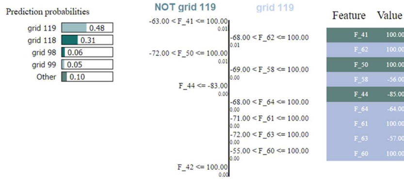
Fig.4. LIME results for 5GHz Wi-Fi based localization
