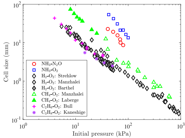
Figure 3: Comparison of the cell width as a function of P_1 for detonation propagating in NH 3 -O 2 , NH 3 -N 2 O, H 2 -O 2 , CH 4 -O 2 , C 2 H 6 -O 2 , and C 3 H 8 -O 2 mixtures. \phi=0.5 for mixtures with NH 3 -N 2 O and \phi=1 for all other mixtures; T_1=293-295 K. References: [48, 49, 50, 51, 52, 53].
