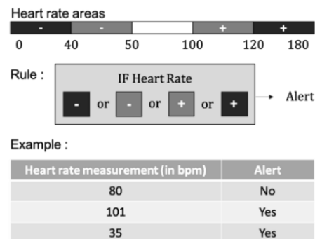
Fig. 5. Example of a rule used in Smart Angel checking the patient's heart rate.
