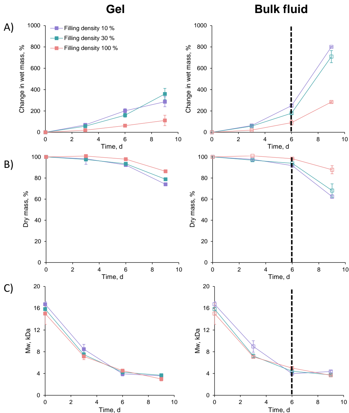
Figure 6: Dynamic changes in the A) wet mass (%), B) dry mass (%), and C) PLGA polymer molecular weight ( M_w ) of the implants upon exposure to agarose gels (left hand side) or well agitated phosphate buffer pH 7.4 (right hand side) (the experimental set-ups are shown in Figure 2) ( n = 3 , mean values \pm SD).
