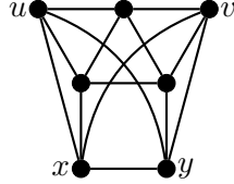
Figure 5: The graph H_7 satisfies \tau(H_7) = 1183 > 1001 = \lceil f(H_7) \rceil .
