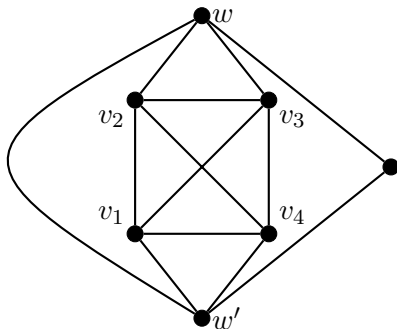
Figure 3: The graph H_4 satisfies \tau(H_4) = 575 > 422 = \lceil f(H_4) \rceil .
