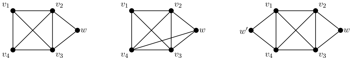
Figure 1: The graphs X_5 (left), X'_5 (middle) and X_6 (right). We have \tau(X_5) = 40 , \tau(X'_5) = 75 and \tau(X_6) = 100 .
