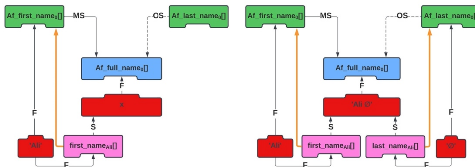
Figure 4: a) Violation of F-slot-companys ; b) A reformulation of the theory with empty informational entities
