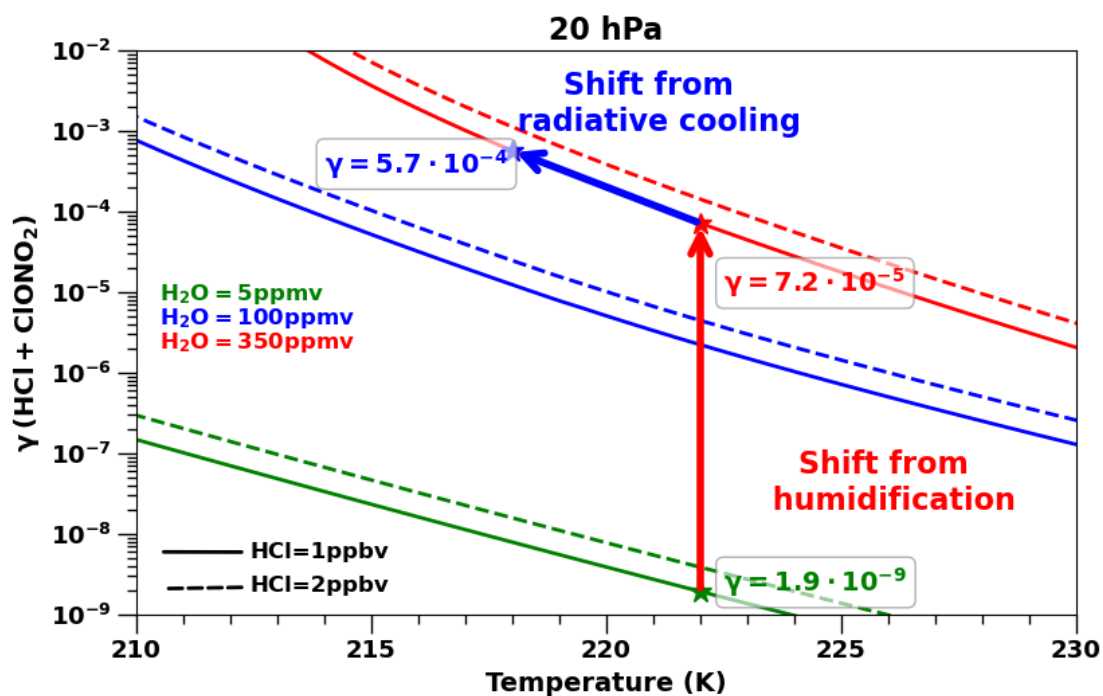
Fig. S2. \gamma values for \text{HCl} + \text{ClONO}_2 in the stratosphere as a function of temperature between 210 and 230 K at 20 hPa, aerosol radius 0.3 \mu\text{m} , and \text{H}_2\text{O} of 5 ppmv (green), 100 ppmv (blue) and 350 ppmv (red), HCl of 1 ppbv (solid line) and 2 ppbv (dashed line) and 0.5 ppbv of \text{ClONO}_2 . The red arrow indicates the shift in \gamma values from humidification from 5 to 350 ppmv and the blue arrow indicates the shift in \gamma values from a -4 \text{ K} radiative cooling.
