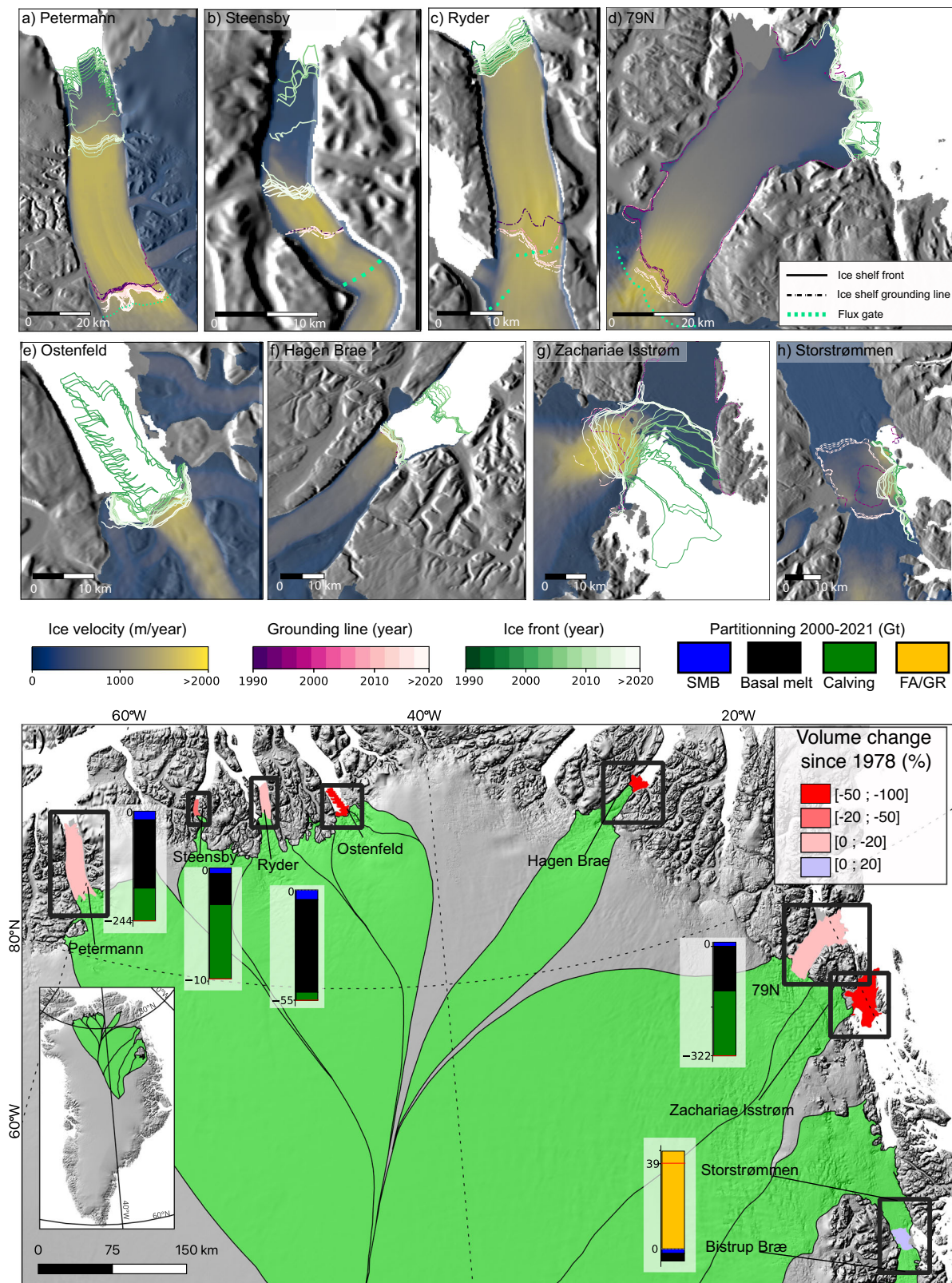
Fig. 1 | Ice shelves changes in North Greenland. Changes in ice shelf frontal and grounding line position between 1990 and present (a–h). Ice flow velocity (source: 4 ) is color coded on a linear color scale and overlaid on a shaded version of the digital elevation model from Bedmachine v3 12 (a–h). i Location of all ice shelves in North Greenland with their maximum extent over the study period. Partitioning is shown as bar plot for the period 2001–2021, with Surface Mass Balance (SMB) in blue, basal melting in black and calving in green. The total cumulative mass budget
