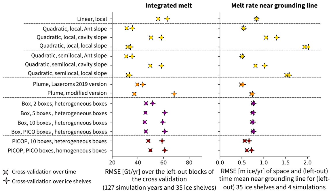
Figure 7. Summary of the RMSE of the integrated melt ( \text{RMSE}_{\text{int}} ) for the cross-validation over time ( \times ) and for the cross-validation over ice shelves ( + ) for a selection of parameterisations, using the 50 km domain (in gigatonnes per year) (left, same as Fig. 4 left), and summary of the RMSE of the melt rate averaged over time and space near the grounding line (average in the first box of the five-box setup, \text{RMSE}_{\text{GL}} ) (in metres of ice per year) (right). The colours represent the different parameterisation approaches: simple (yellow), plume (orange), box (purple), and PICOP (brown). The RMSE is computed following Eq. (33, left panel) and Eq. (35, right panel) on the synthetically independent evaluation dataset. “Ant slope” stands for “Antarctic slope”.
