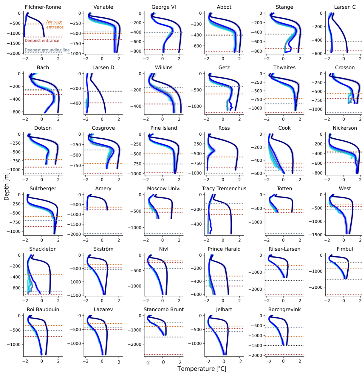
Figure 3. Comparison of mean input temperature profiles between the five different domains which were averaged (10, 25, 50, 100 km, and offshore) in one given simulation (REALISTIC). The shading represents the interannual variability (1 standard deviation over time). The horizontal dotted lines show the average depth of the bed at the ice front (light brown), the largest depth of the bed at the ice front (dark brown), and the largest depth of the grounding line (grey). For a few ice shelves, the deepest entrance is deeper than 1500 m depth, but the profiles are defined over the continental shelf (depth shallower than -1500 m). A black dotted line denotes the 1500 m limit in this case. For Stange and Larsen C ice shelves, the average entrance depth and the deepest grounding line overlap.
