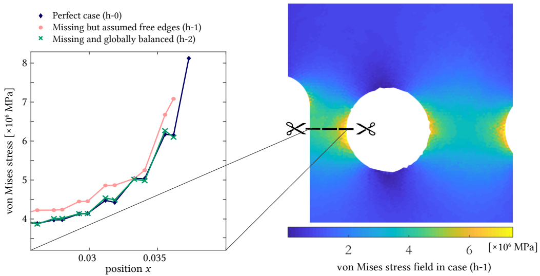
Figure 9: von Mises stress field (right) and reported values along a horizontal line going through the sample (left), for the three cases.
