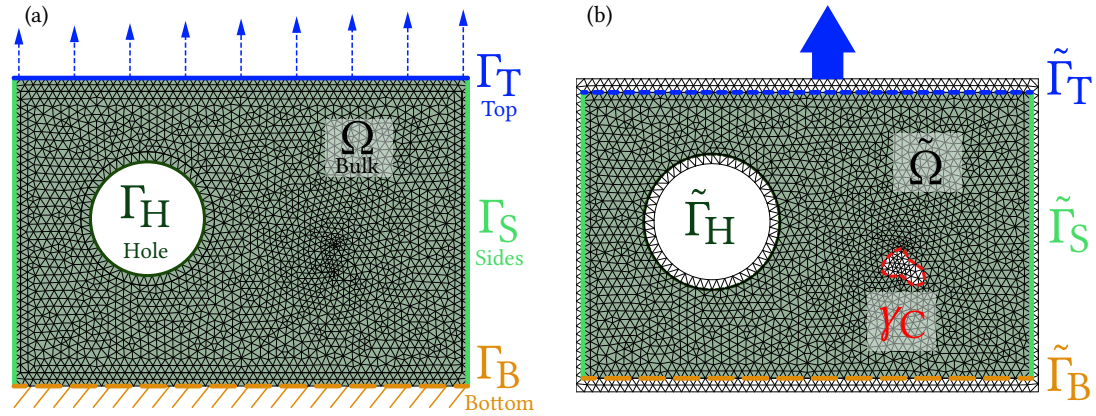
Figure 1: Problem formulation: (a) theoretical and (b) real problems with three particular modified boundaries: top boundary with grip, cluster of missing data and imperfectly defined edges close to hole.
