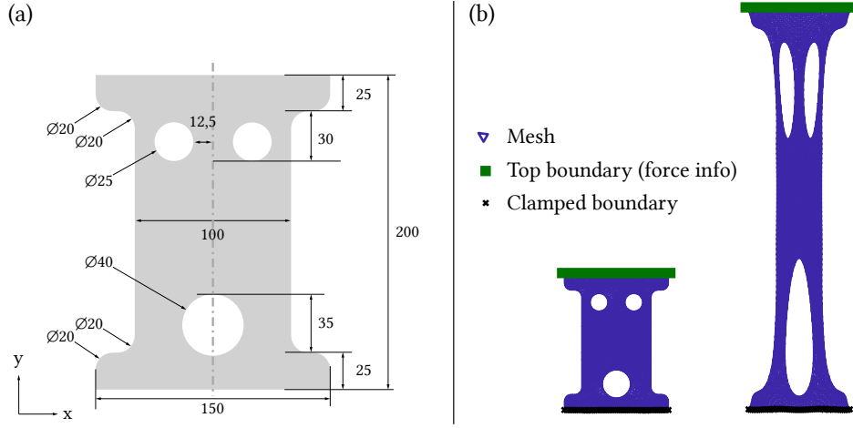
Figure 3: Case study of a perforated hyperelastic membrane under uniaxial tension: (a) initial geometry, (b) mesh after 200 % of total macroscopic strain. On the top nodes, information on force is available while the bottom ones are clamped.
