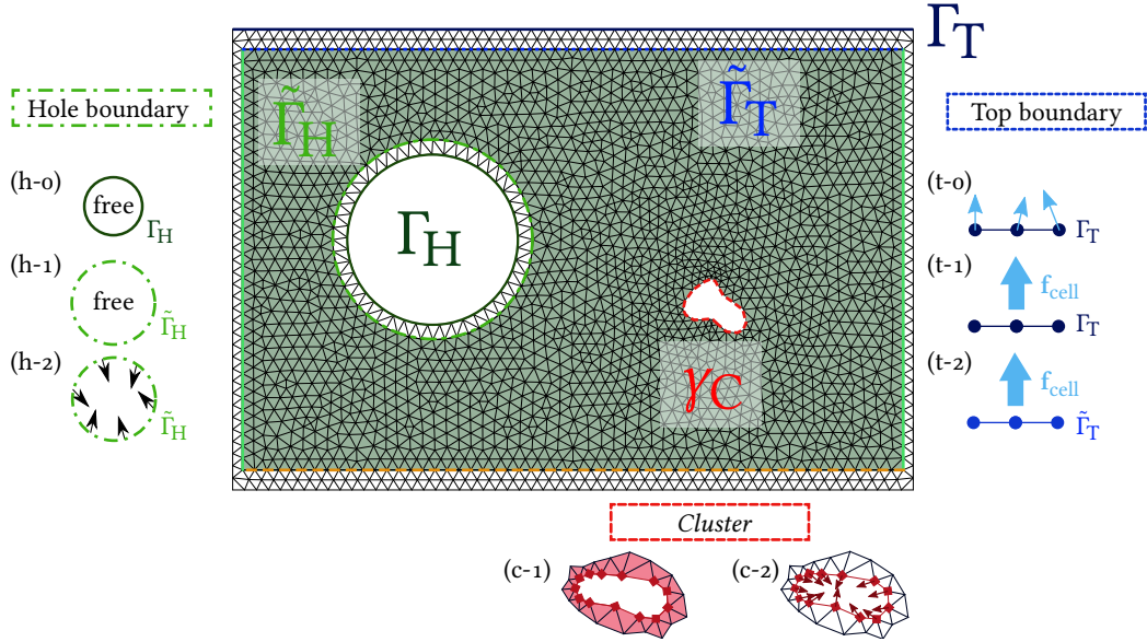
Figure 2: Summary of the possible preprocessing choices. They concern missing data for three particular boundaries: top boundary with grip, cluster of missing data and imperfectly defined edges close to hole.
