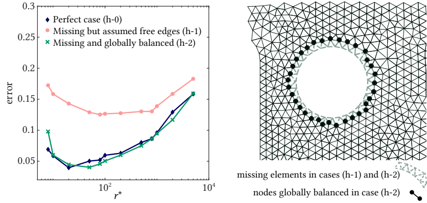
Figure 8: Influence of preprocessing choice for the hole edge definition on the error as a function of r^* for a given C , for the cases of an imperfectly defined edge close to the hole (with (h-1) the assumption of free edge, (h-2) the global balance condition) and of a perfectly defined edge (h-0) (left subfigure). Nodes/elements used in the calculations (right subfigure).
