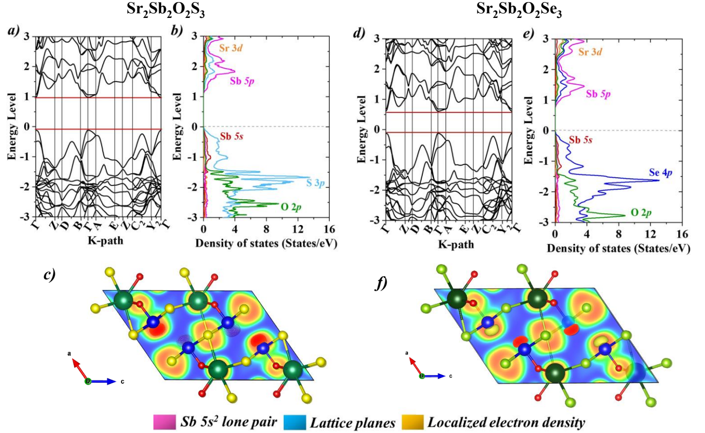
Figure 4 : (a) and (d) Electronic band structure, (b) and (e) Projected DOS is shown for the Sr 3d, Sb 5s, Sb 5p, S 3p/ Se 4p and O 2p states. The Fermi level is set to 0, (c) and (f) Local electron density projected on the (010) lattice plane and 0.91 isosurface levels of DFT plots of Sr 2 Sb 2 O 2 S 3 and Sr 2 Sb 2 O 2 Se 3 , respectively, for the P2 1 /c model.
